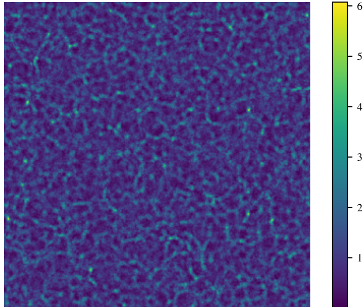
Fig. 16. Example scintillation pattern generating from propagating the phase screen from Fig. 6 containing atmospheric turbulence over 10km.
