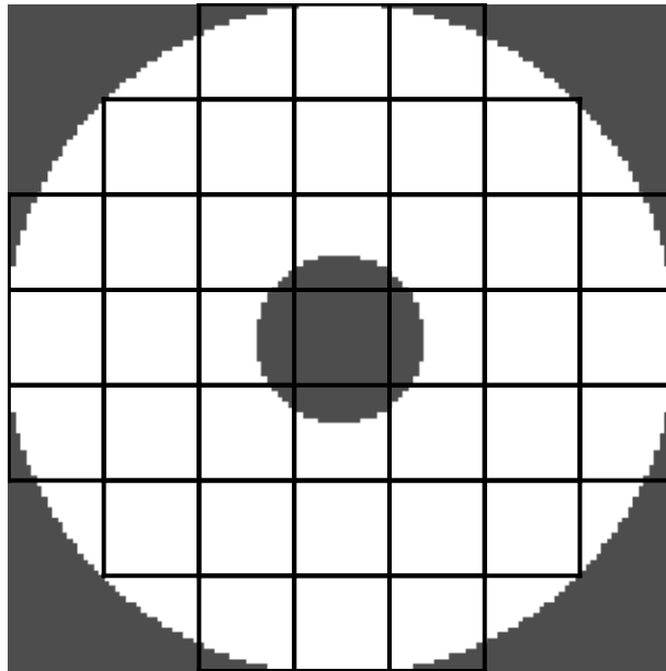
Fig. 13. Calculation of WFS sub-apertures with a given fill factor or higher for the pupil defined in Fig. 1. This allows for the creation of masks which can be applied to WFS data to remove measurements from sub-apertures which do not receive enough light to generate useful data. This can be used to filter WFS data from simulations and RTCs, removing noisy data.
