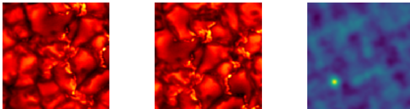
Fig. 12. The left and middle images show the reference image and a shifted sub-aperture image of solar granulation respectively. The right most image shows the correlation image created from the cross-correlation of the left and center images. This can then be centroided in order to measure the shift between the sub-aperture image and the reference image.
