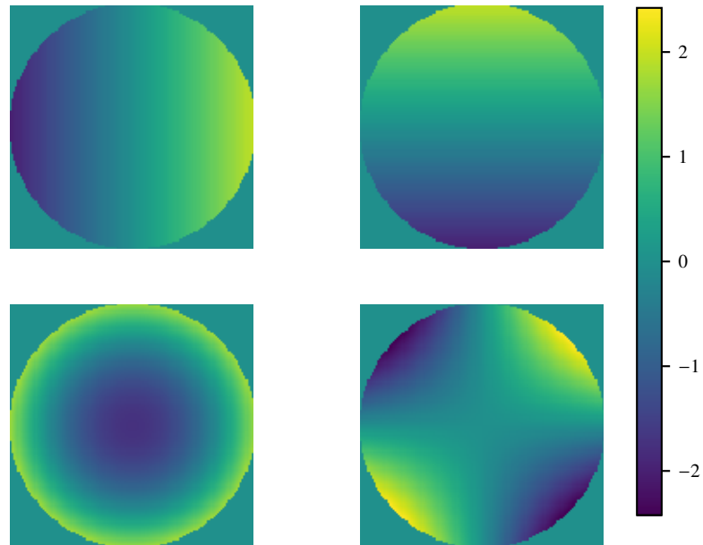
Fig. 4. The first four Zernike modes (excluding piston) generated using the example code shown in Fig. 3.
