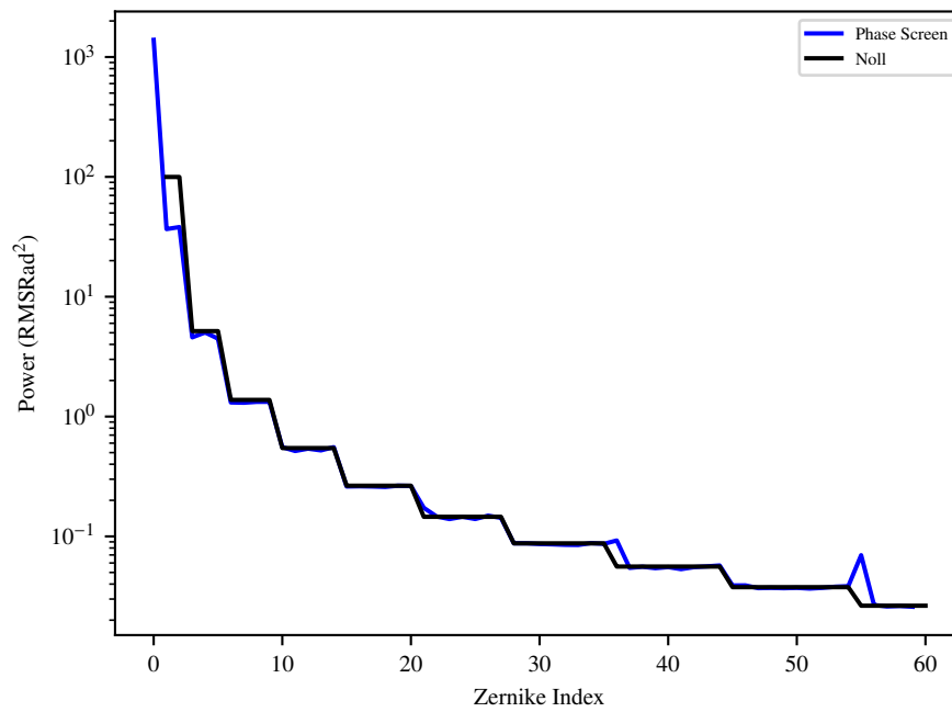
Fig. 7. The average Zernike breakdown of 1000 individual Fried infinite phase screens [15,16], with the theoretical strengths expected from Noll [12].
