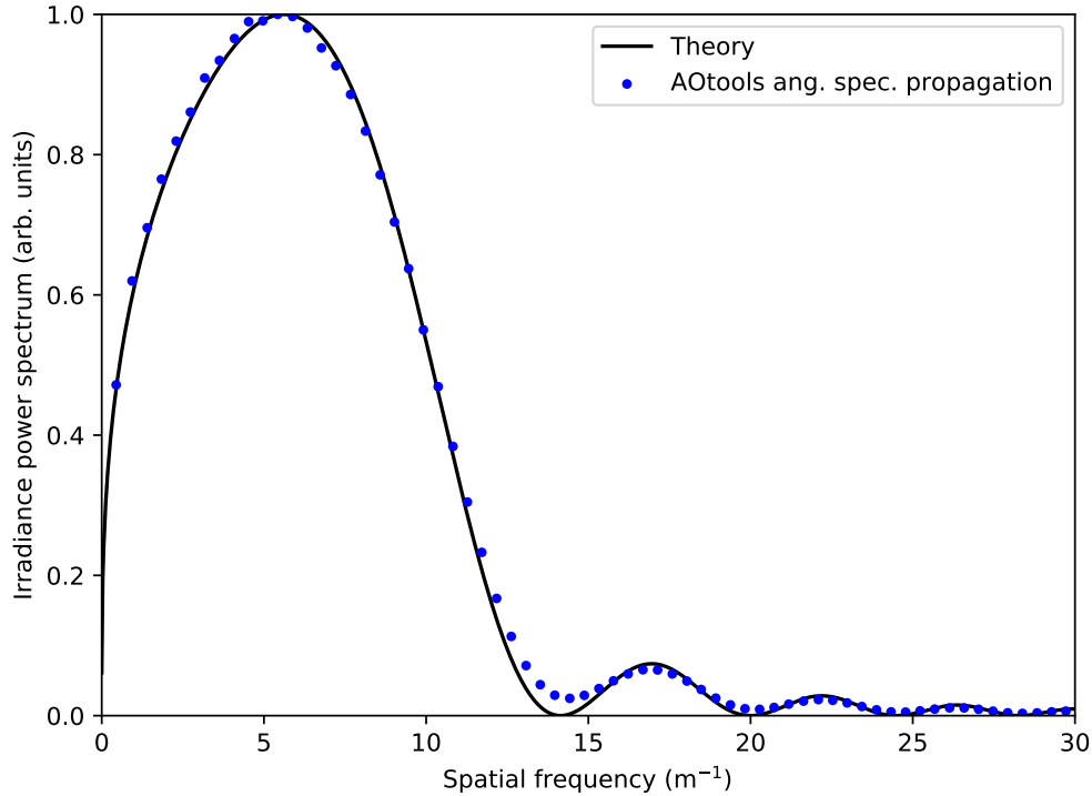
Fig. 17. Scintillation irradiance power spectrum obtained by using AOtools angular spectrum propagation to propagate 500 phase screens a distance of 10 km. Each screen has r_0 = 32 cm.
