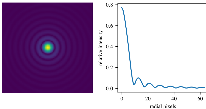
Fig. 9. PSF corresponding to the pupil shown in Fig. 2 along side the the corresponding azimuthal average of the PSF calculated using AOtools.
