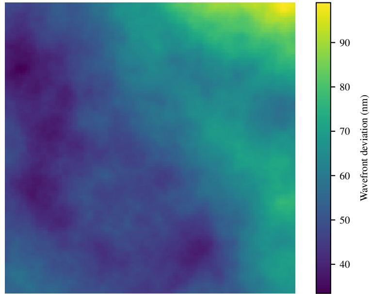
Fig. 6. Example phase screen generated using the Fried infinite phase screen method [15,16] using the code shown in Fig. 5. The strengths is defined in nm such that the phase screen is wavelength in dependant.
