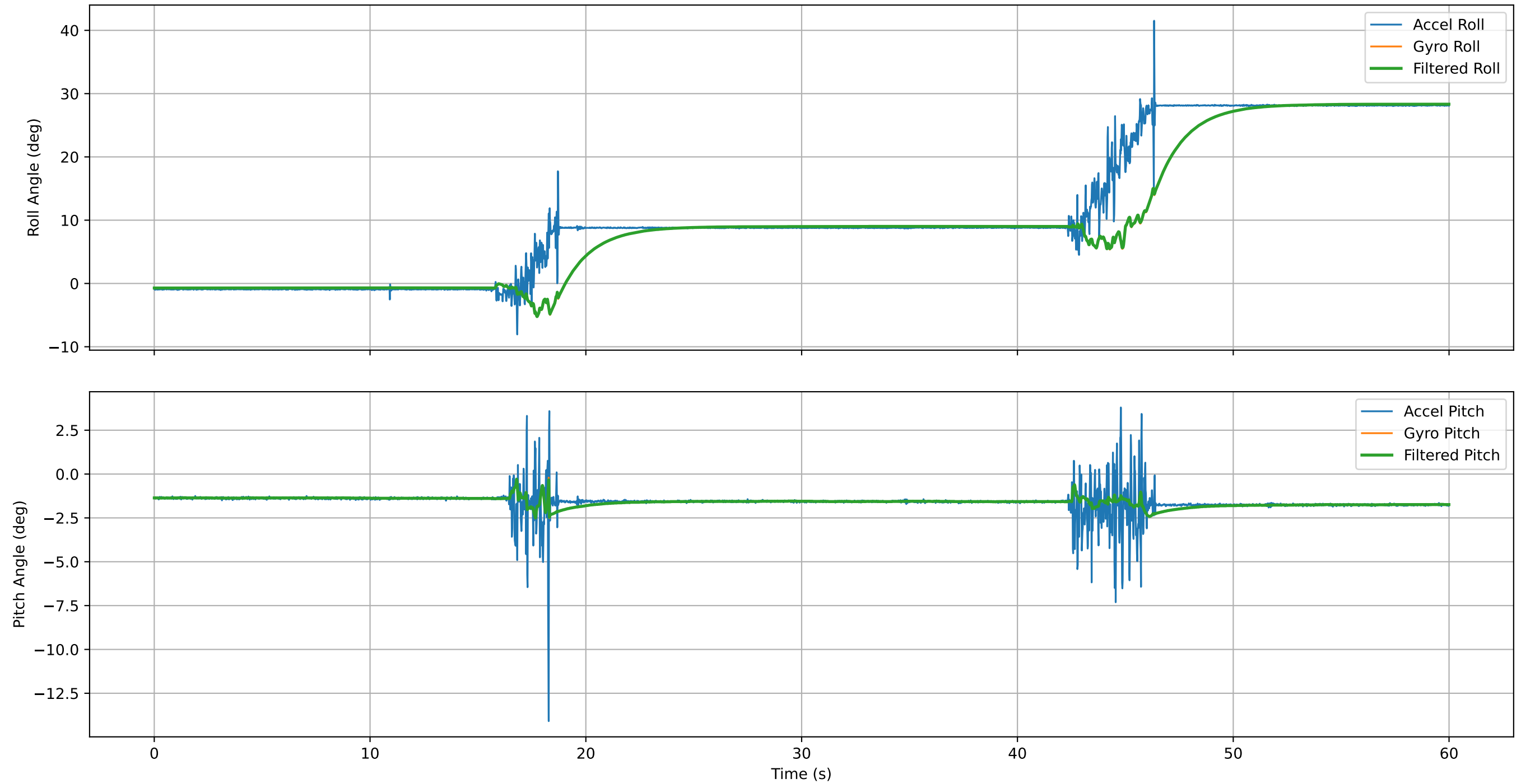
Complementary Filter Angles After 60 s
