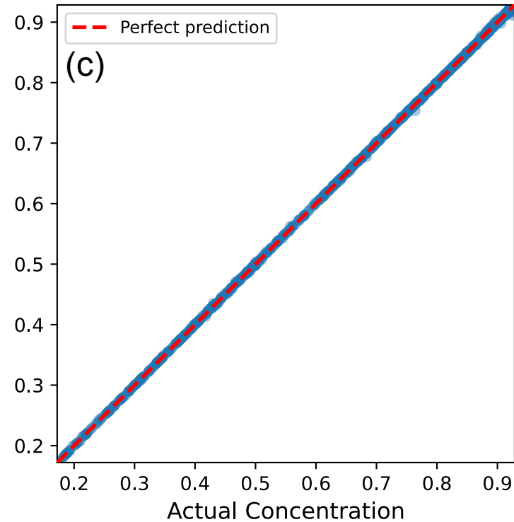
PINN_AB, RMSE = 0.0015
