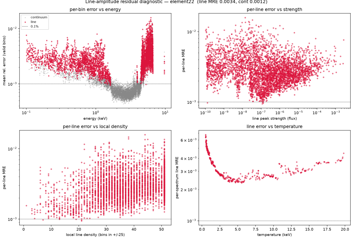
Figure 1: Per-line amplitude residual for titanium ( Z = 22 , production line head; zinc is qualitatively identical). Clockwise from top left: per-bin relative error versus energy (line bins red, continuum grey – the continuum dips below the 0.1% dotted line mid-band); per-line error versus line strength (flat – the error is carried neither by the weak nor the strong lines); per-spectrum line MRE versus temperature (U-shaped, worst at the coldest T ); and per-line error versus local line density (a weak secondary trend). The dominant feature is a uniform \sim 0.3\% floor immune to line strength, with a cold-temperature excess on top.
