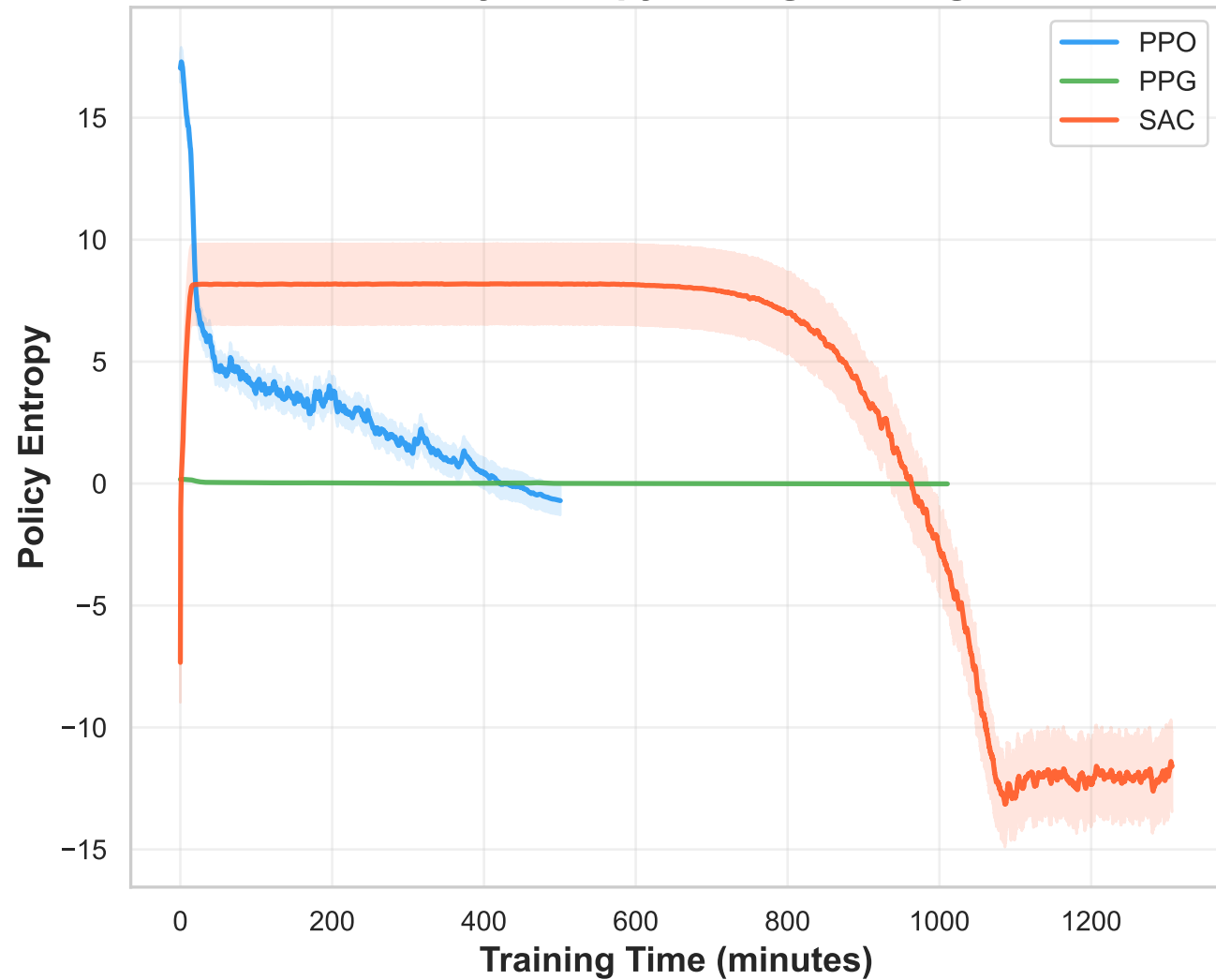
Policy Entropy During Training
