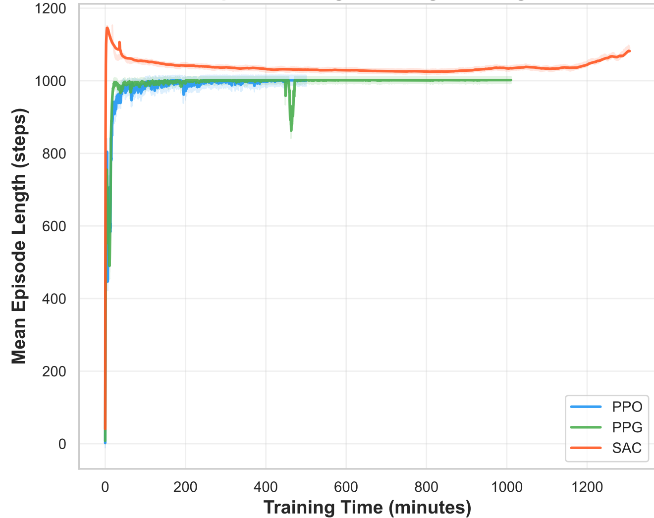
Episode Length During Training
