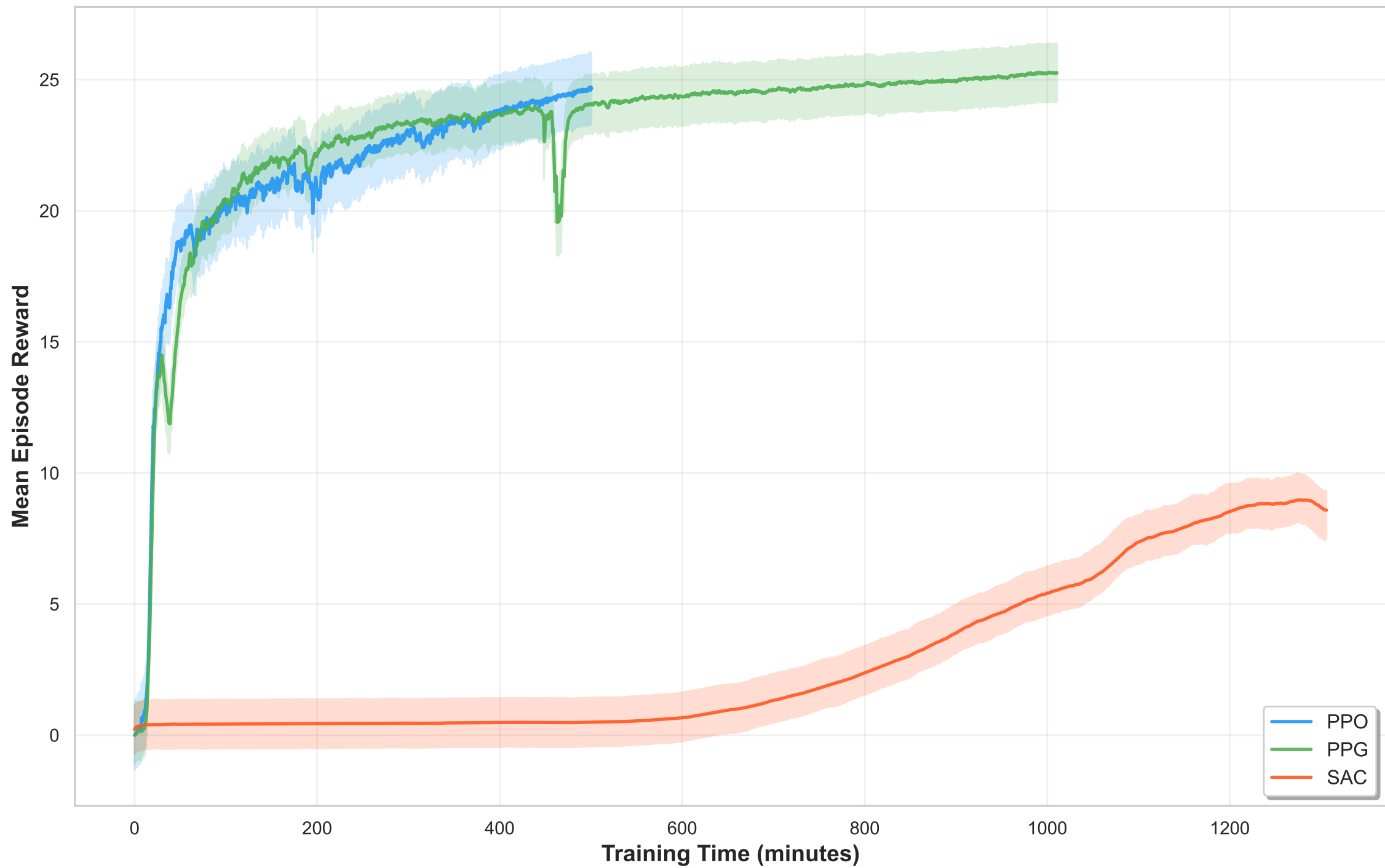
Training Curves: PPO vs PPG vs SAC
