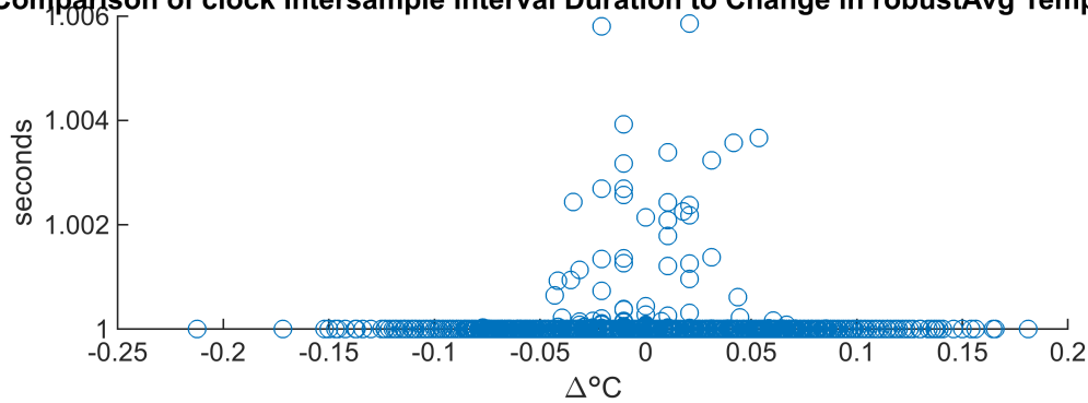
Comparison of clock Intersample Interval Duration to Change in robustAvg Temperature
