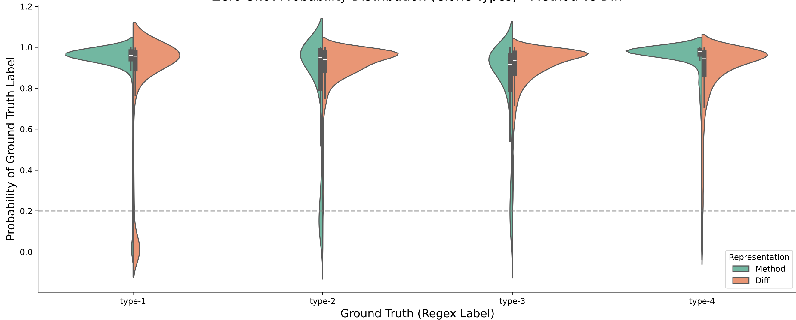
Zero-Shot Probability Distribution (Clone Types) - Method vs Diff
