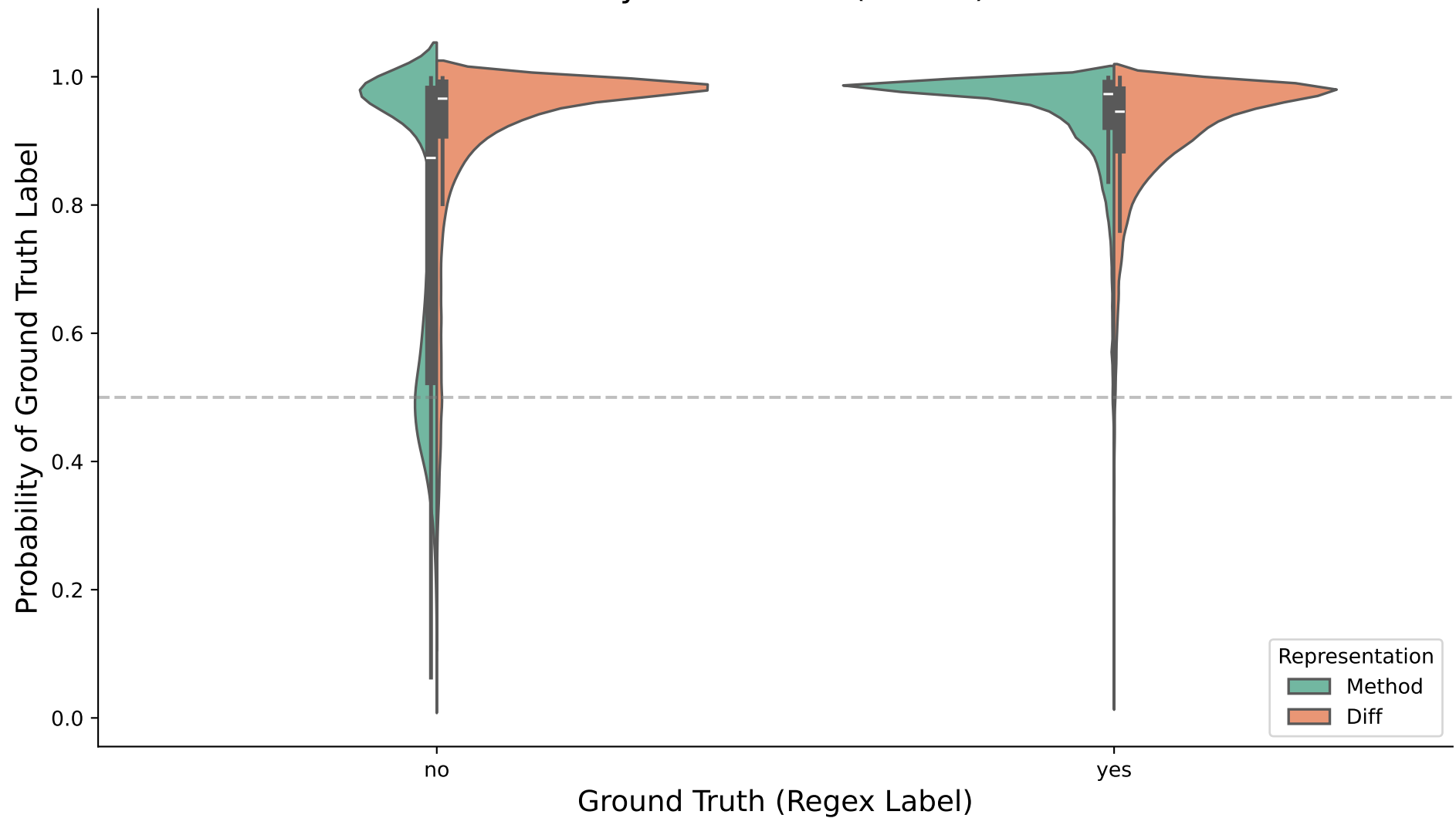
Zero-Shot Probability Distribution (Yes/No) - Method vs Diff
