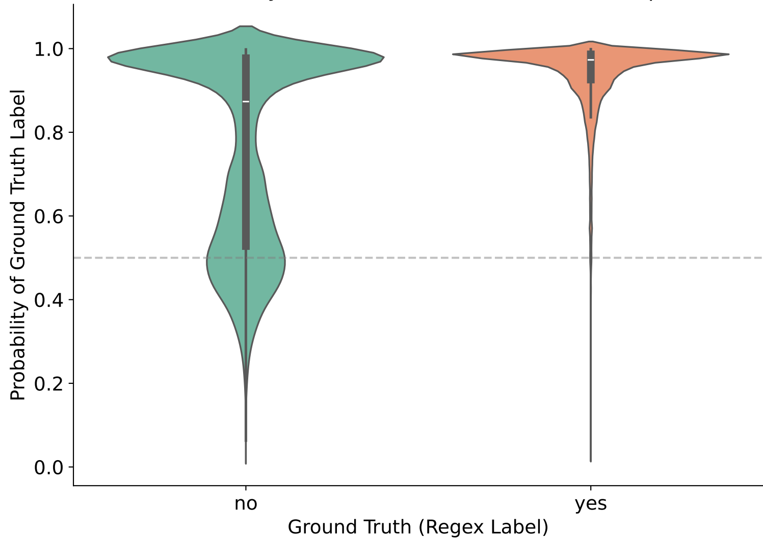
Zero-Shot Probability Distribution (Yes/No) - Method Representation
