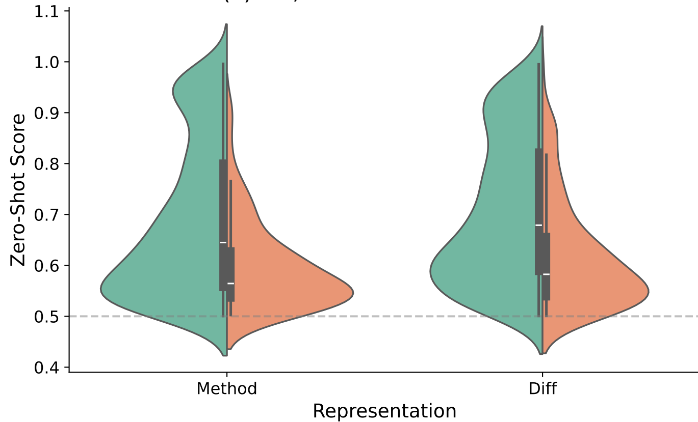
(a) Yes/No Classification Tasks
