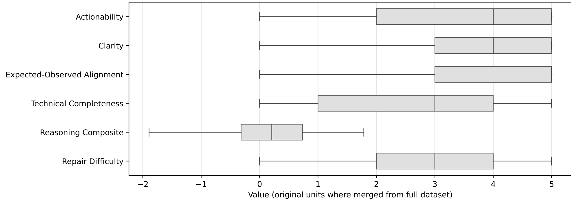
Feature distribution — LLM-Assessed Semantic Quality
