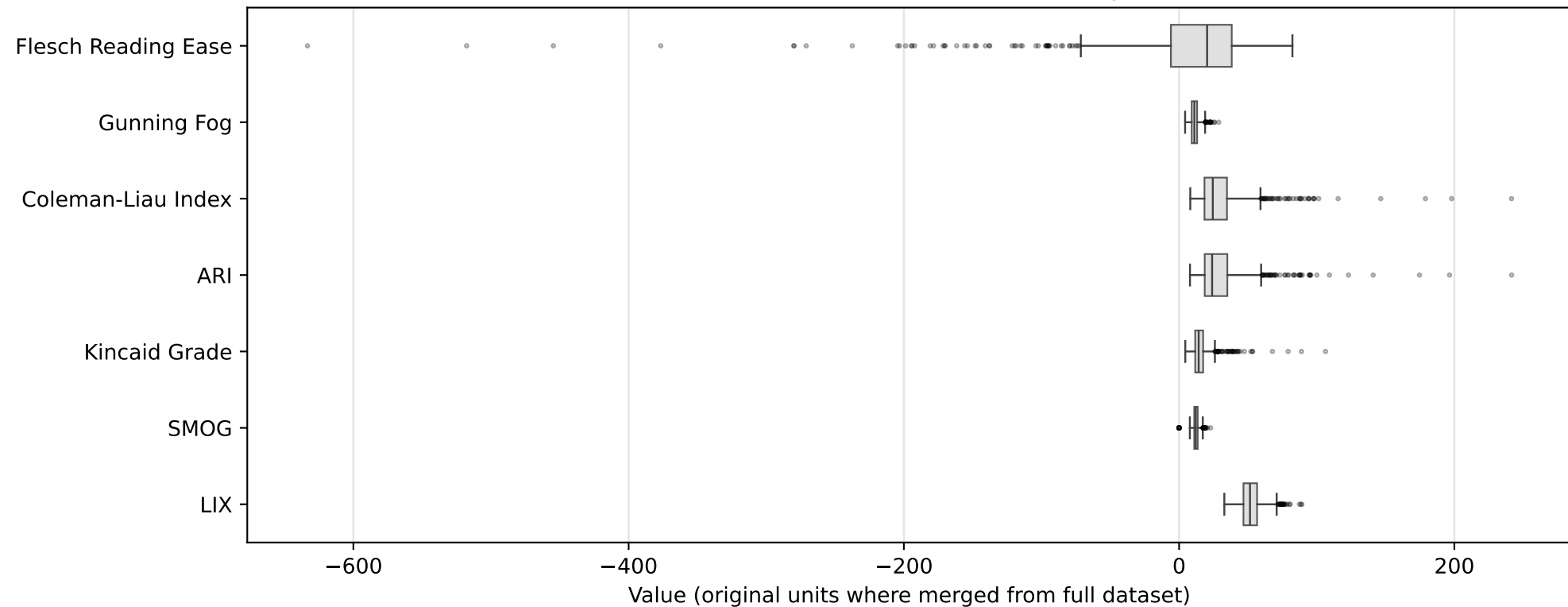
Feature distribution — Readability
