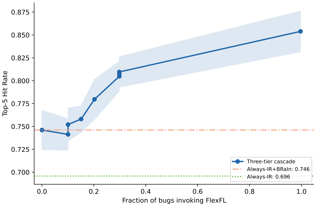
Three-Tier Cascade — Top-5 Hit Rate (IR → BRain → FlexFL, 5-fold CV)
