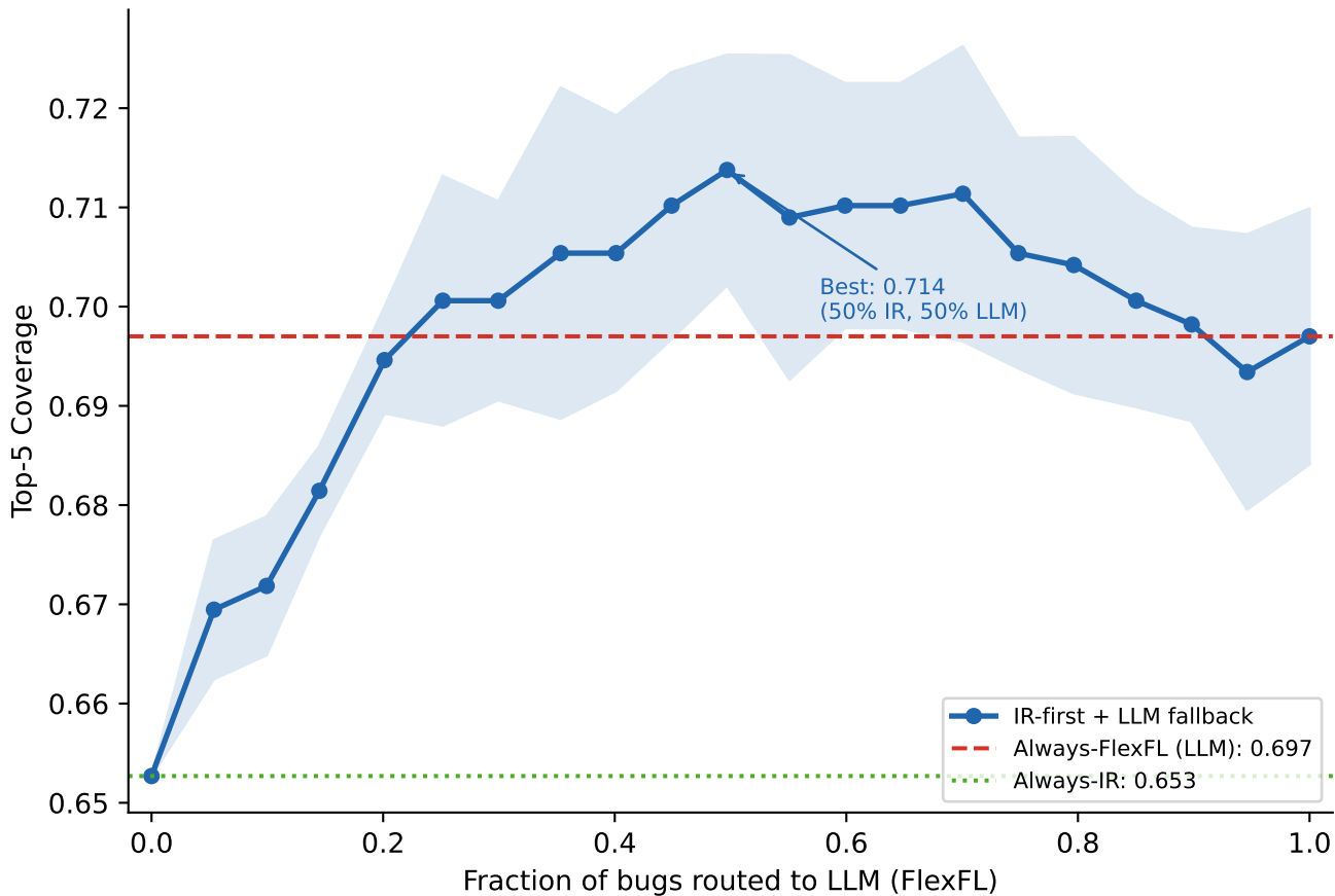
Cost-Coverage Tradeoff: IR-first with LLM Fallback
