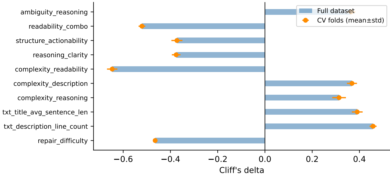
Delta stability — BugLocator (Top-5)
