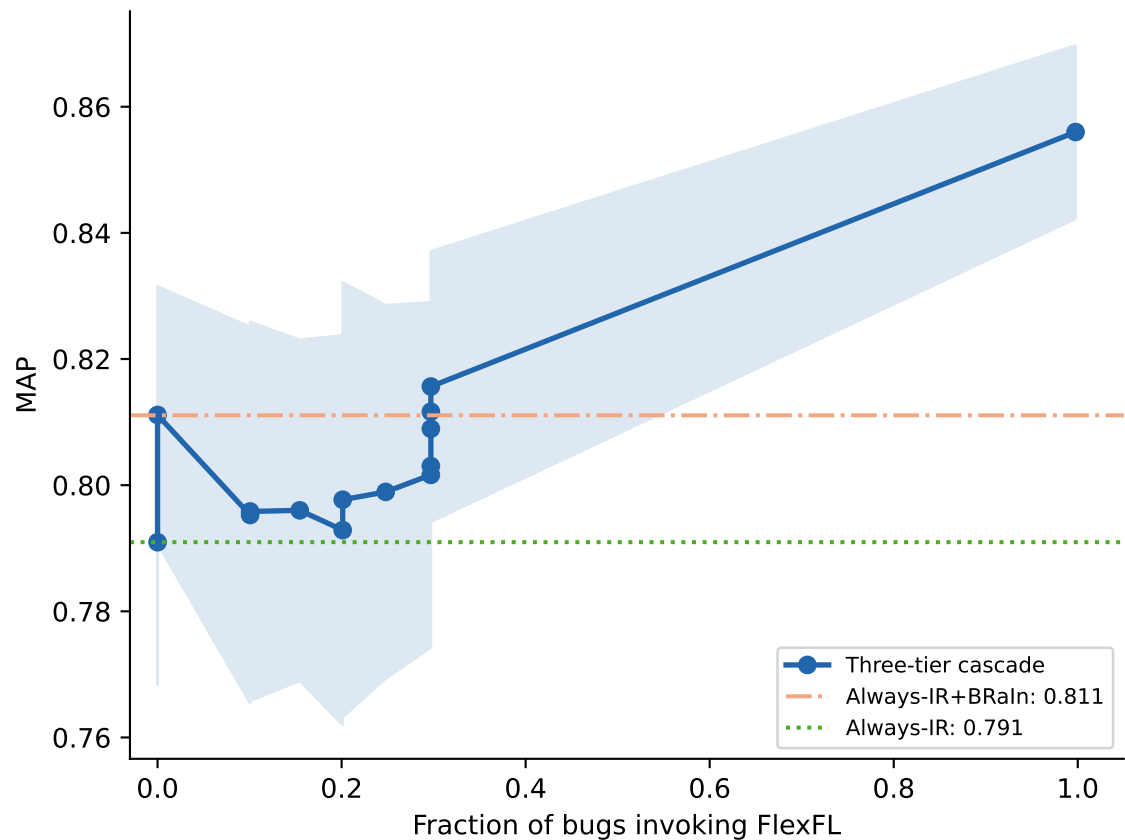
Three-Tier Cascade — MAP (IR → BRain → FlexFL, 5-fold CV)
