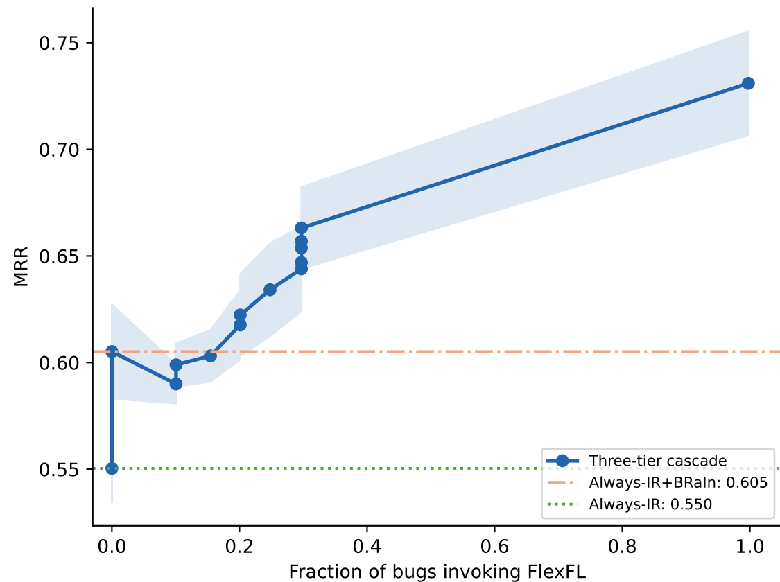
Three-Tier Cascade — MRR (IR → BRain → FlexFL, 5-fold CV)
