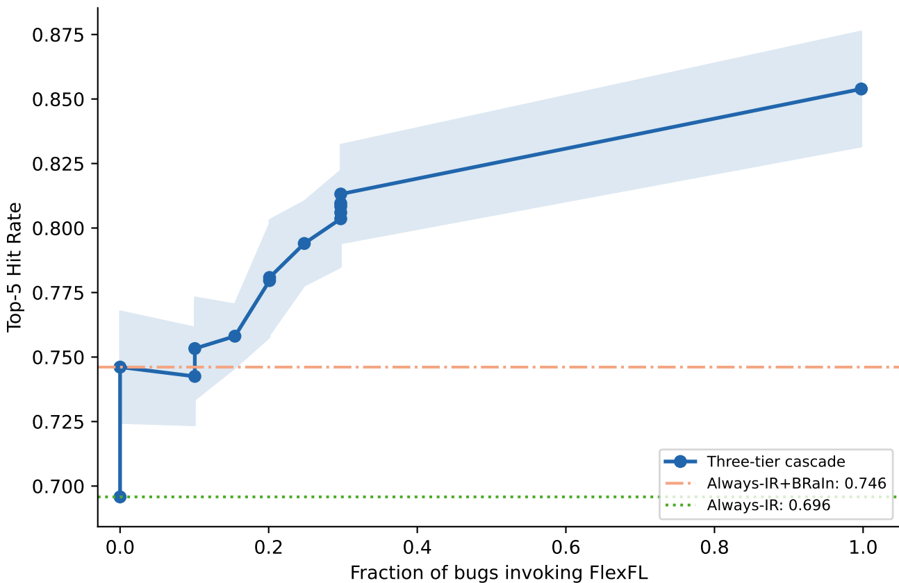
Three-Tier Cascade — Top-5 Hit Rate (IR → BRaln → FlexFL, 5-fold CV)
