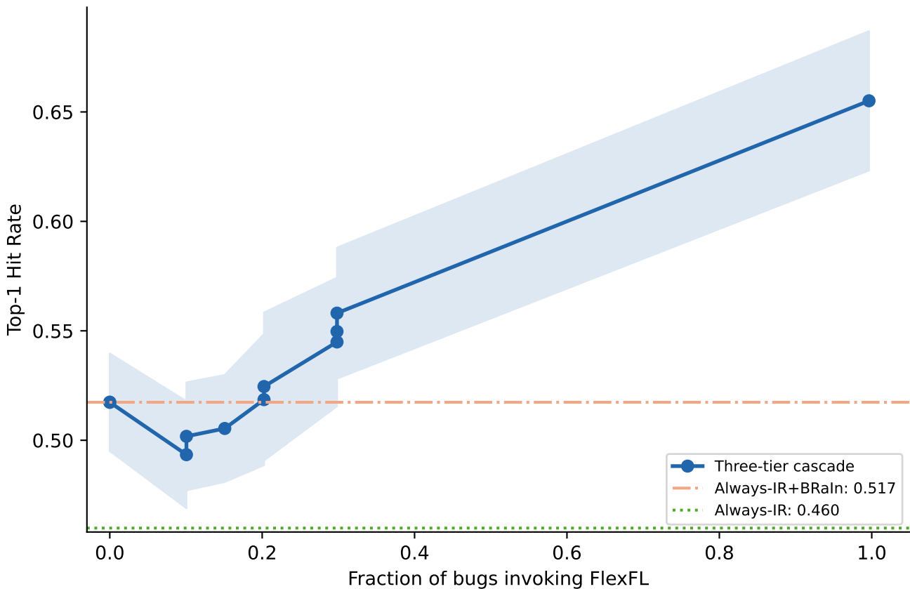
Three-Tier Cascade — Top-1 Hit Rate (IR → BRain → FlexFL, 5-fold CV)
