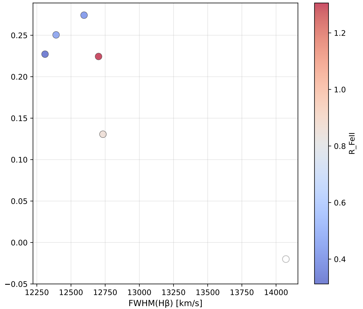
ALERCE fid=1 (N=5 det, 1 non-det)
