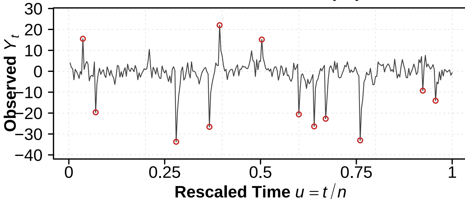
Innovation Outliers (IO)
