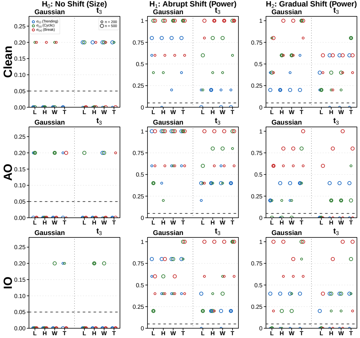
Figure 1: Empirical rejection rates for robust location change-point tests under ARMA(2,1) dependence. Evaluated under H_0 (size), H_1 (abrupt break at u = 0.5 ), and H_2 (gradual linear change) with shift magnitude \delta = 0.5 at nominal level \alpha = 0.05 (dashed line). Rows represent Clean, AO, and IO with \varepsilon = 0.05 scenarios for Gaussian and Student- t_3 errors. Methods: L (Proposed Linearized Welsch CUSUM), H (Huberized CUSUM; ?), W (Wilcoxon test; ?), and T (Hodges–Lehmann test; ?). Circle colors represent variance scenarios: smooth trending (blue), cyclic (green), and abrupt break (red). Open circle markers scale with sample size n \in \{200, 500, 1000\} .
