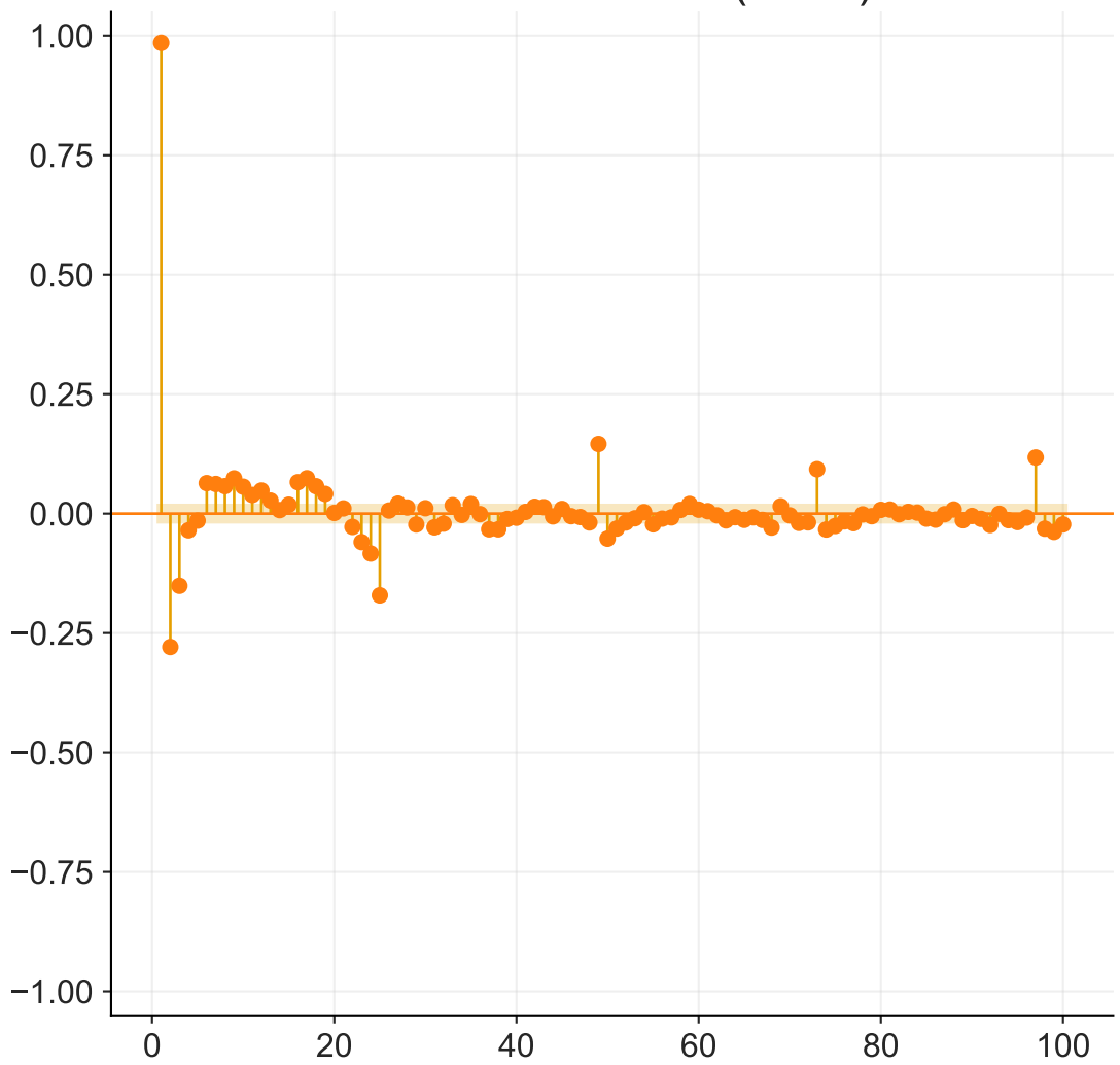
PACF Emissions (2021)
