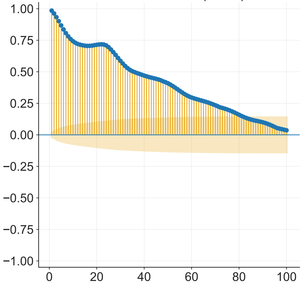
ACF Emissions (2021)
