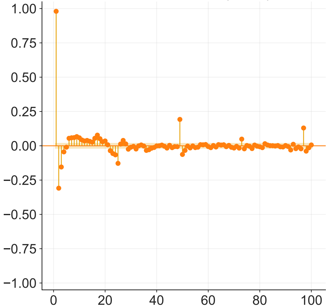
PACF Emissions (2020)
