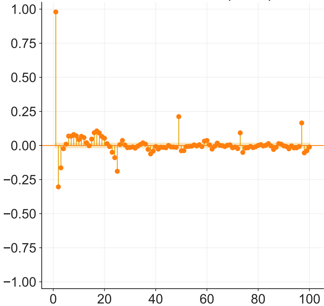
PACF Generation (2019)
