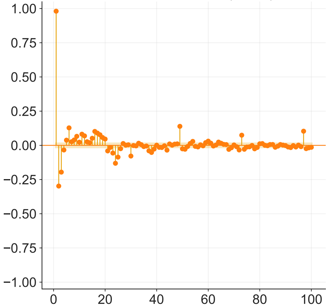
PACF Generation (2022)
