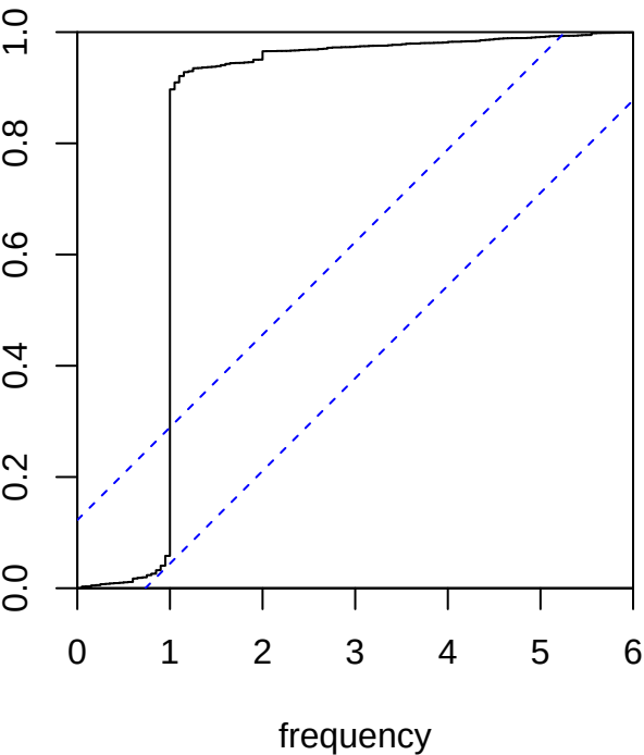
Series: nottem
