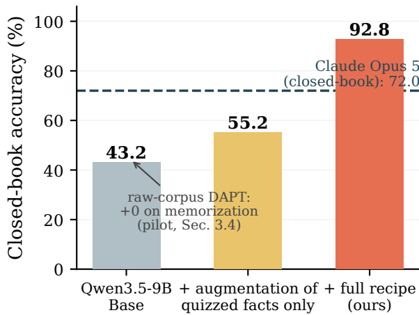
Figure 1. The recipe, not the corpus, carries the result. Closed-book accuracy on the 125-question layered audit set. Continued pretraining on the raw 31M-token corpus leaves memorization at base level despite halving training loss (pilot measurement, §3.4); augmenting only the quizzed facts helps only those facts (55.2%); the full recipe—coverage of all facts, 24 diverse templates, reversed forms, whole-table narratives—reaches 92.8%, surpassing Claude Opus 5 (dashed line).
