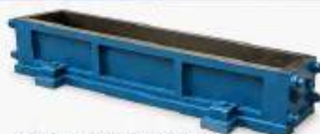
100 mm x 100 mm x 500 mm Beam Mould (Cast Iron)
