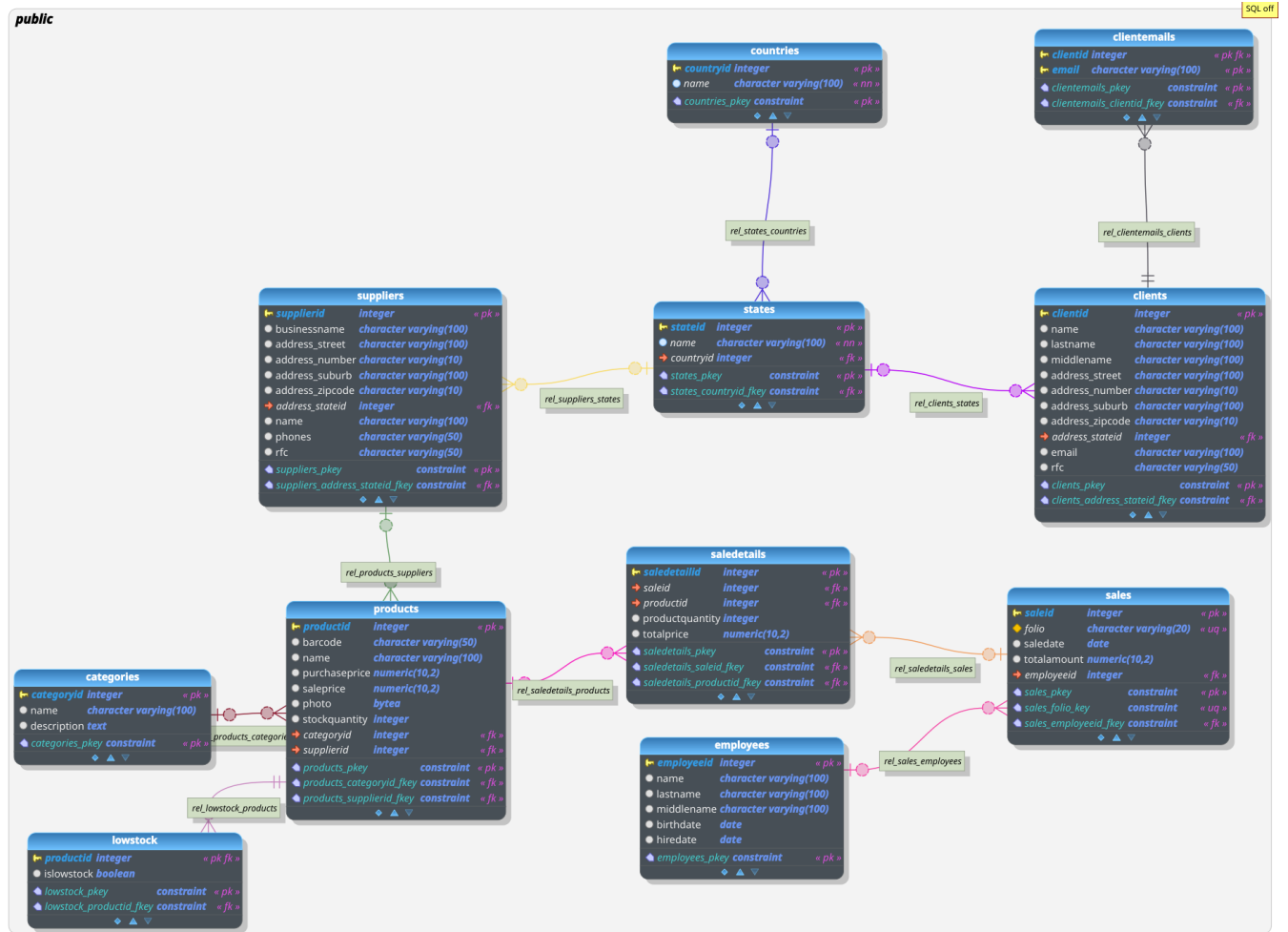
Figura 2.2: Relational Model of our case study
