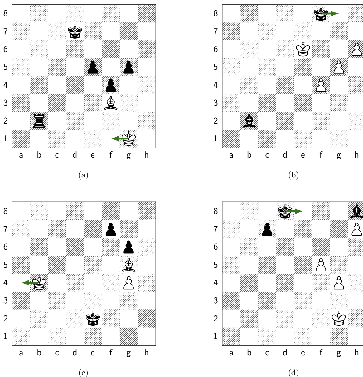
Figure 62: Move 68, White: Kf1 . (a) Our position; Melanie plays Kf1 (g1f1). Panels (b)–(d) are the retrieved master positions whose correspondence most drove this move (highest QAP objective among those that transfer to it). (b) Retrieved from ccr1_top_p0003#2424 (ply 119) [structural distance d=4 , QAP obj=2]: the master played Kg8; under \mu our Kg1 plays the role of that game’s Kf1; cross-type roles: our rb2 as their ph6; transferred move g1f1 ( endorses this move ). (c) Retrieved from ccr1_top_p0001#1531 (ply 150) [structural distance d=11 , QAP obj=2]: the master played Ka4; under \mu our Kg1 plays the role of that game’s Kb4; transferred move g1f1 ( endorses this move ). (d) Retrieved from ccr1_top_p0000#1437 (ply 121) [structural distance d=10 , QAP obj=2]: the master played Ke8; under \mu our Kg1 plays the role of that game’s Kd1; cross-type roles: our rb2 as their Pc7; transferred move g1f1 ( endorses this move ). Synthesis: 18 retrieved analogs transferred to Kf1 (summed QAP objective 27, the strongest correspondence among the candidate moves); Melanie committed it via the search selector.
