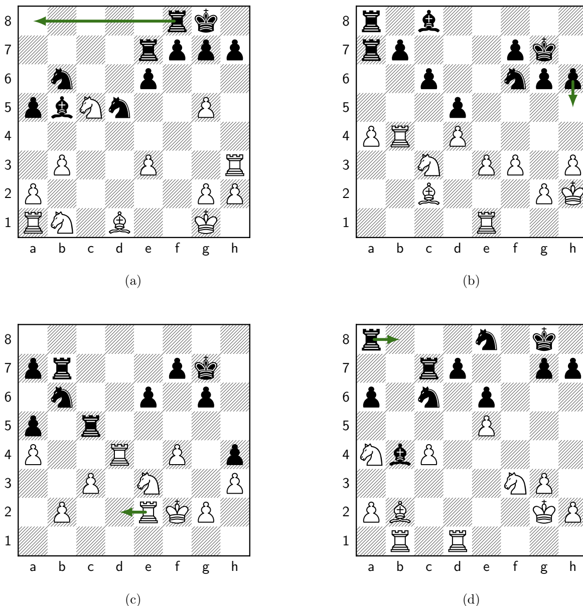
Figure 22: Move 28, Black: Ra8 (f8a8) . (a) Our position; Melanie plays Ra8 (f8a8). Panels (b)–(d) are the retrieved master positions whose correspondence most drove this move (highest QAP objective among those that transfer to it). (b) Retrieved from ccr1_top_p0003#2650 (ply 67) [structural distance d=64 , QAP obj=50]: the master played h5; under \mu our Rf1 plays the role of that game’s Ph3 (a cross-type correspondence); cross-type roles: our rh3 as their Bc8 , our Nd5 as their Ra7 ; transferred move f8a8 ( endorses this move ). (c) Retrieved from ccr1_top_p0000#3626 (ply 60) [structural distance d=63 , QAP obj=43]: the master played Red2; under \mu our Rf1 plays the role of that game’s Re2 ; cross-type roles: our Bb5 as their Pg2 , our Re7 as their Ne3 ; transferred move f8a8 ( endorses this move ). (d) Retrieved from ccr1_top_p0000#1318 (ply 47) [structural distance d=57 , QAP obj=30]: the master played Rb8; under \mu our Rf1 plays the role of that game’s Ra1 ; cross-type roles: our Pf7 as their Ne8 , our Nb6 as their Rc7 ; transferred move f8a8 ( endorses this move ). Synthesis: 3 retrieved analogs transferred to Ra8 (summed QAP objective 123, the strongest correspondence among the candidate moves); Melanie committed it via the search selector.
