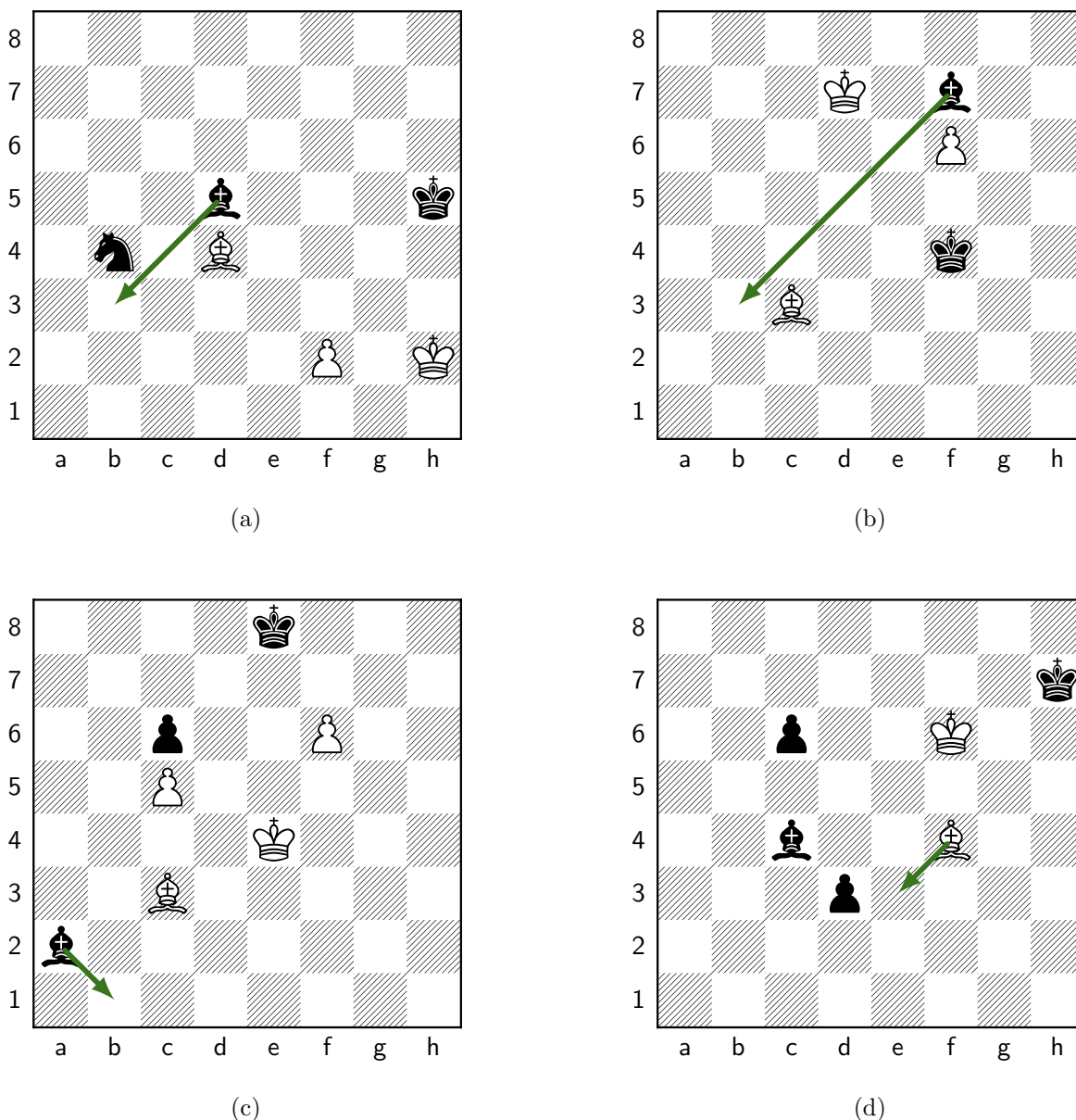
Figure 107: Move 113, Black: Bb3. (a) Our position; Melanie plays Bb3 (d5b3). Panels (b)–(d) are the retrieved master positions whose correspondence most drove this move (highest QAP objective among those that transfer to it). (b) Retrieved from lichess_elite_2024-09_p0020#2804 (ply 229) [structural distance d=6 , QAP obj=1]: the master played Bb3; under \mu our Bd4 plays the role of that game’s Bf2 ; transferred move d5b3 ( endorses this move ). (c) Retrieved from lichess_elite_2024-09_p0022#1319 (ply 221) [structural distance d=11 , QAP obj=1]: the master played Bb1+; under \mu our Bd4 plays the role of that game’s Ba7 ; cross-type roles: our Nb4 as their Pc6 ; transferred move d5b3 ( endorses this move ). (d) Retrieved from lichess_elite_2024-09_p0019#2827 (ply 238) [structural distance d=7 , QAP obj=1]: the master played Be3; under \mu our Bd4 plays the role of that game’s Bf4 ; cross-type roles: our Nb4 as their pc6 ; transferred move d5c4. Synthesis: 4 retrieved analogs transferred to Bb3 (summed QAP objective 3, the strongest correspondence among the candidate moves); Melanie committed it via the search selector.
