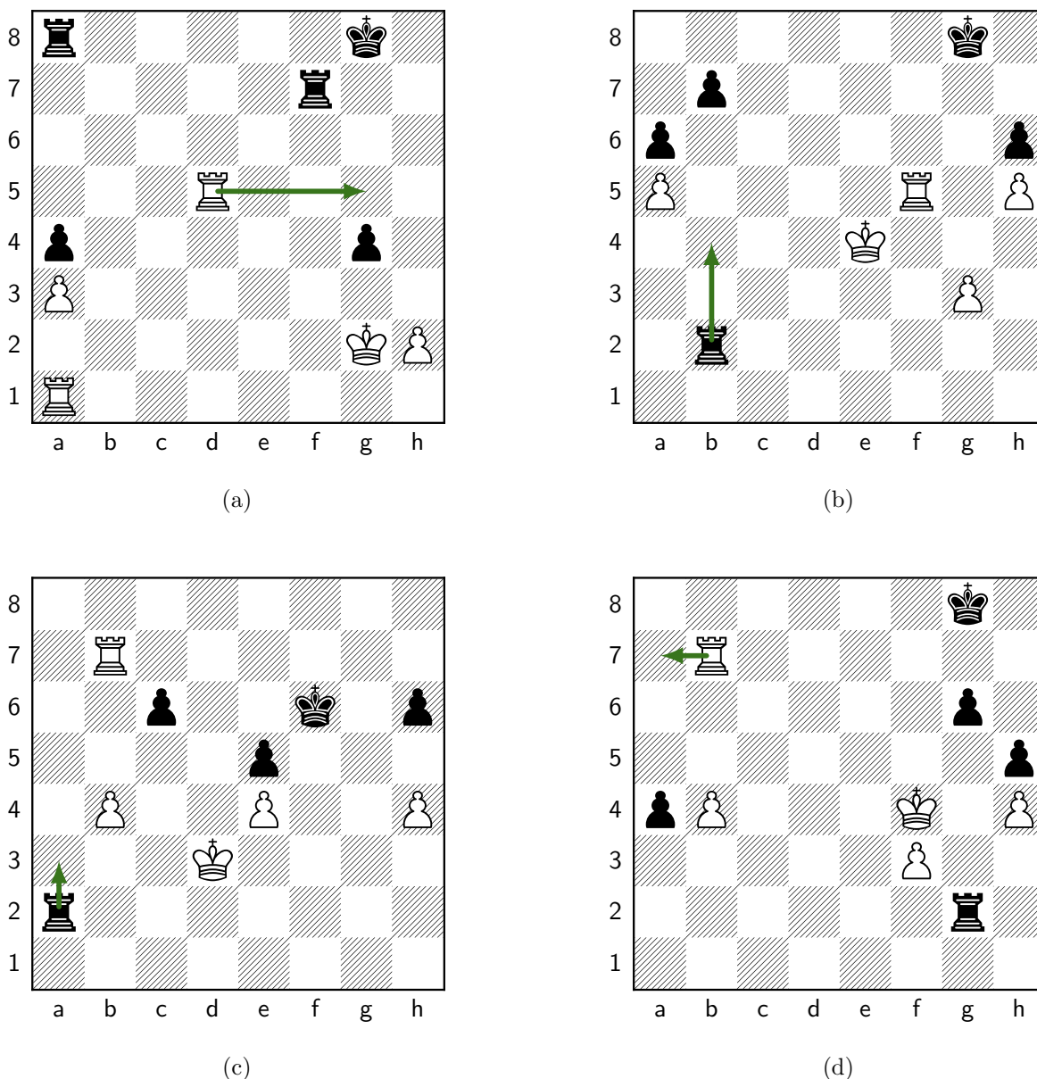
Figure 25: Move 31, White: Rg5+. (a) Our position; Melanie plays Rg5+ (d5g5). Panels (b)–(d) are the retrieved master positions whose correspondence most drove this move (highest QAP objective among those that transfer to it). (b) Retrieved from ccr1_top_p0001#2688 (ply 73) [structural distance d=20 , QAP obj=2]: the master played Rb4+; under \mu our R d5 plays the role of that game’s R b7 ; cross-type roles: our r a8 as their P b7 , our R a1 as their p g3 ; transferred move d5g5 ( endorses this move ). (c) Retrieved from ccr1_top_p0001#3037 (ply 73) [structural distance d=21 , QAP obj=2]: the master played Ra3+; under \mu our R d5 plays the role of that game’s R a7 ; cross-type roles: our R a1 as their P c6 , our r a8 as their p b4 ; transferred move d5g5 ( endorses this move ). (d) Retrieved from ccr1_top_p0001#3184 (ply 72) [structural distance d=19 , QAP obj=1]: the master played Ra7; under \mu our R d5 plays the role of that game’s R b7 ; cross-type roles: our r a8 as their P f3 , our R a1 as their p a4 ; transferred move d5g5 ( endorses this move ). Synthesis: 8 retrieved analogs transferred to Rg5+ (summed QAP objective 10, the strongest correspondence among the candidate moves); Melanie committed it via the search selector.
