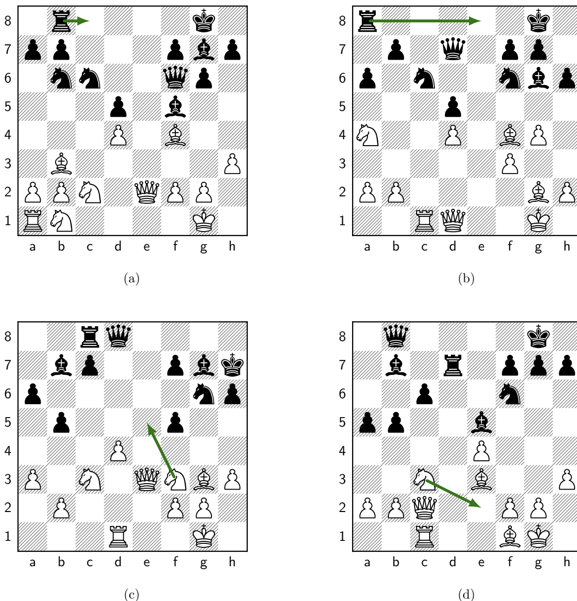
Figure 13: Move 19, Black: Rc8. (a) Our position; Melanie plays Rc8 (b8c8). Panels (b)–(d) are the retrieved master positions whose correspondence most drove this move (highest QAP objective among those that transfer to it). (b) Retrieved from ccr1_top_p0003#1491 (ply 35) [structural distance d=95 , QAP obj=38]: the master played Re8; under \mu our Rb1 plays the role of that game's Ra1; cross-type roles: our Bg7 as their Pg7, our qe2 as their Pa6; transferred move b8c8 ( endorses this move ). (c) Retrieved from ccr1_top_p0000#3146 (ply 42) [structural distance d=83 , QAP obj=38]: the master played Ne5; under \mu our Rb1 plays the role of that game's Nf3 (a cross-type correspondence); cross-type roles: our Nb6 as their Rd1, our Nc6 as their Pf2; transferred move b8c8 ( endorses this move ). (d) Retrieved from ccr1_top_p0000#3091 (ply 40) [structural distance d=88 , QAP obj=27]: the master played Ne2; under \mu our Rb1 plays the role of that game's Nc3 (a cross-type correspondence); cross-type roles: our Qf6 as their Rc1, our Pf7 as their Bf1; transferred move b8c8 ( endorses this move ). Synthesis: 3 retrieved analogs transferred to Rc8 (summed QAP objective 103, the strongest correspondence among the candidate moves); Melanie committed it via the search selector.
