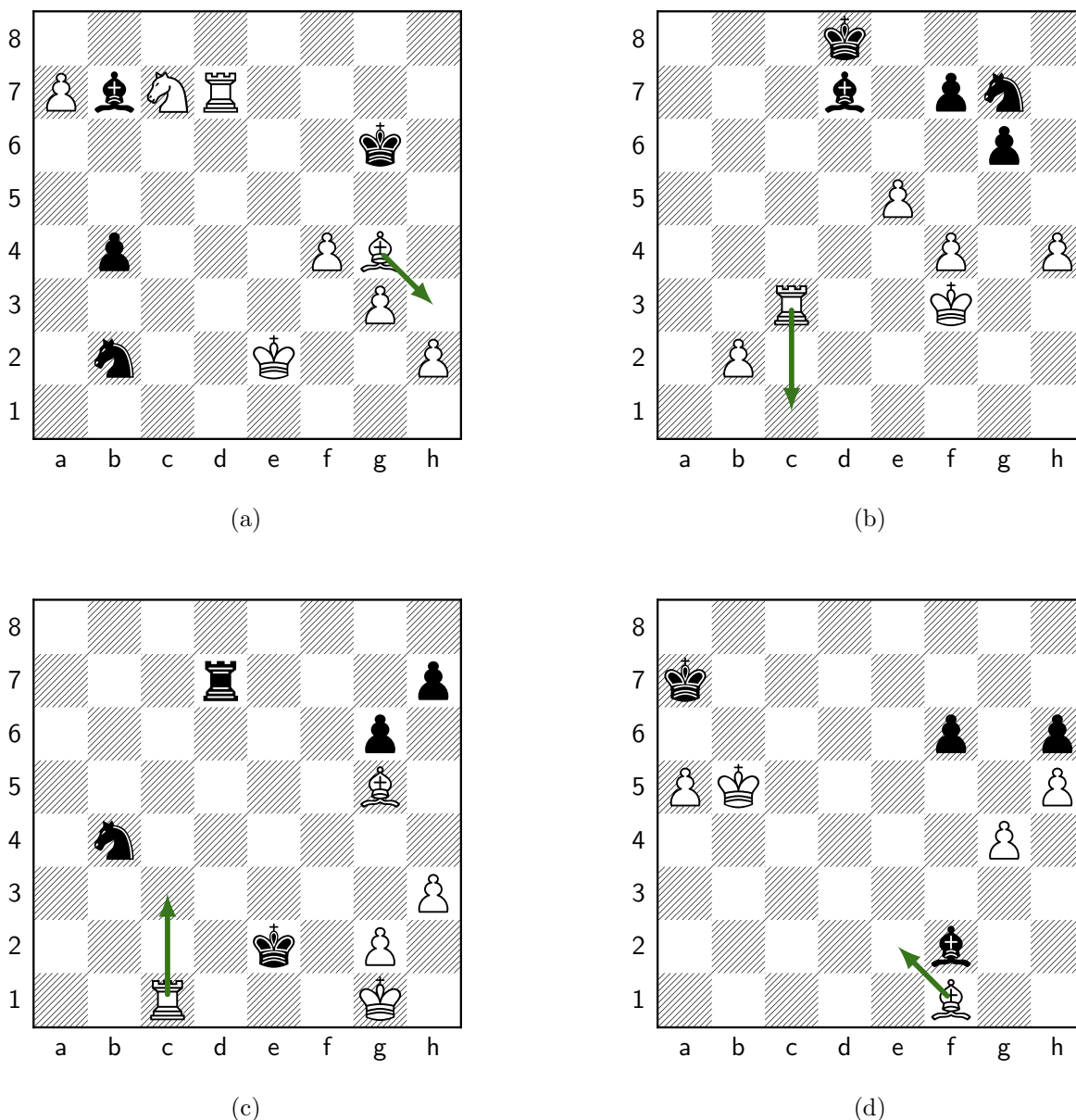
Figure 70: Move 76, White: Bh3 . (a) Our position; Melanie plays Bh3 (g4h3). Panels (b)–(d) are the retrieved master positions whose correspondence most drove this move (highest QAP objective among those that transfer to it). (b) Retrieved from ccr1_top_p0003#523 (ply 146) [structural distance d=36 , QAP obj=3]: the master played Rc1; under \mu our Bg4 plays the role of that game's Rc3 (a cross-type correspondence); cross-type roles: our nb2 as their Pb2, our Nc7 as their Pf4; transferred move g4h3 ( endorses this move ). (c) Retrieved from ccr1_top_p0002#779 (ply 152) [structural distance d=40 , QAP obj=3]: the master played Rc3; under \mu our Bg4 plays the role of that game's Rc1 (a cross-type correspondence); cross-type roles: our Nc7 as their Ph3, our Pg3 as their nb4; transferred move g4h3 ( endorses this move ). (d) Retrieved from ccr1_top_p0002#834 (ply 152) [structural distance d=42 , QAP obj=2]: the master played Be2; under \mu our Bg4 plays the role of that game's Bf1; cross-type roles: our nb2 as their bf2, our bb7 as their Pg4; transferred move g4h3 ( endorses this move ). Synthesis: 4 retrieved analogs transferred to Bh3 (summed QAP objective 10, the strongest correspondence among the candidate moves); Melanie committed it via the search selector.
