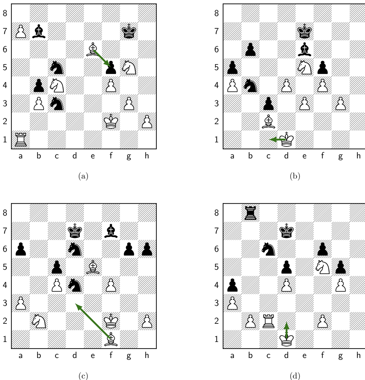
Figure 53: Move 59, White: Bxf5. (a) Our position; Melanie plays Bxf5 (e6f5). Panels (b)–(d) are the retrieved master positions whose correspondence most drove this move (highest QAP objective among those that transfer to it). (b) Retrieved from ccr1_top_p0001#3939 (ply 110) [structural distance d=57 , QAP obj=38]: the master played Kc1; under \mu our Kf2 plays the role of that game’s Kd1; cross-type roles: our bb7 as their pc3, our Ng5 as their Pg3; transferred move f2g1. (c) Retrieved from ccr1_top_p0000#3032 (ply 114) [structural distance d=62 , QAP obj=36]: the master played Bd3; under \mu our Pg3 plays the role of that game’s Bf1 (a cross-type correspondence); cross-type roles: our pb4 as their Nb2, our nc3 as their Pa3; transferred move g3g4. (d) Retrieved from ccr1_top_p0002#3150 (ply 100) [structural distance d=59 , QAP obj=33]: the master played Kd2; under \mu our Kf2 plays the role of that game’s Kd1; cross-type roles: our nc5 as their Rc2, our bb7 as their Pf2; transferred move f2f1. Synthesis: no retrieved analog transferred to Bxf5 – the search selector chose it on value (material / mate); panels (b)–(d) show the strongest nearby analogies.
