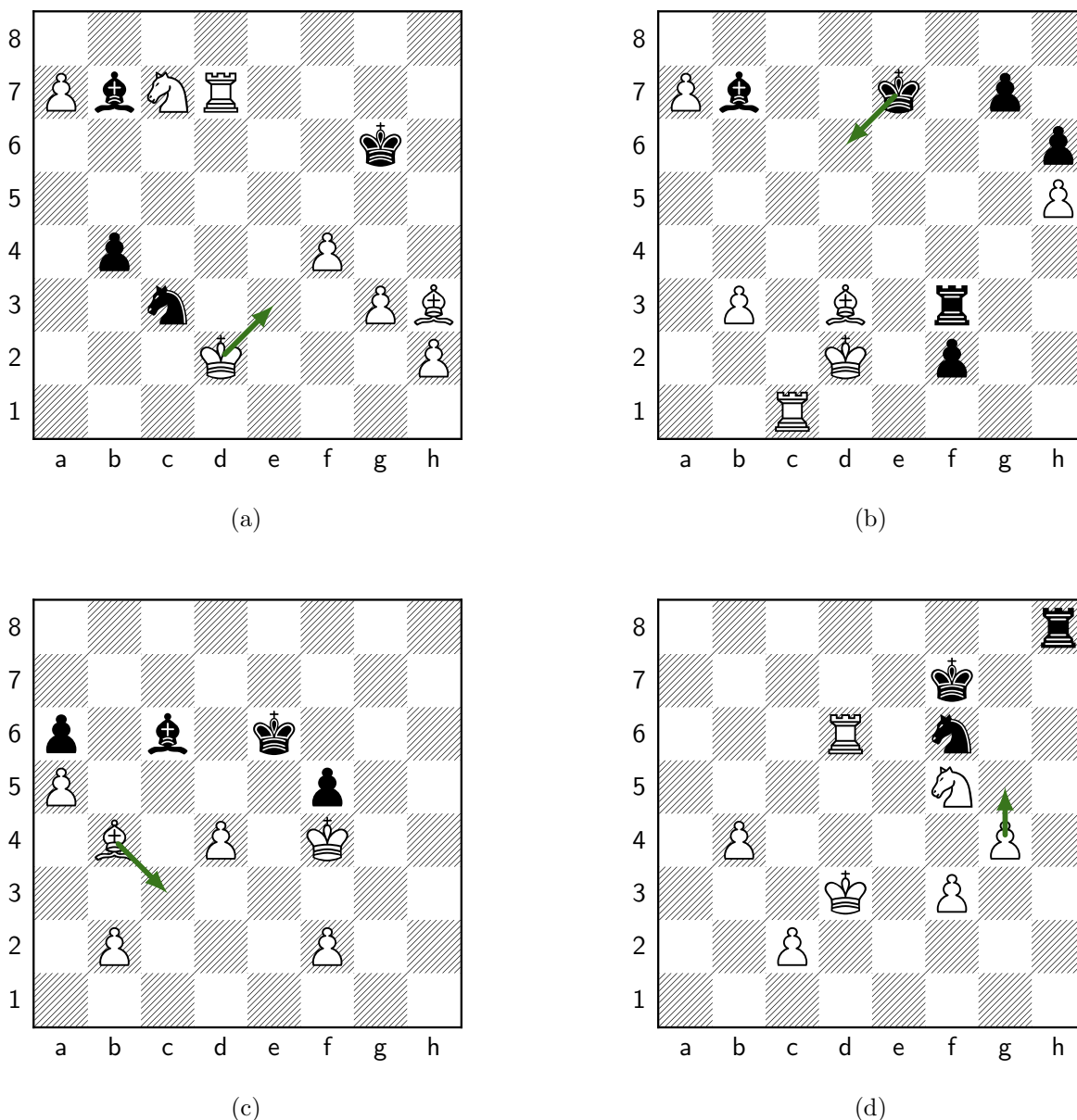
Figure 74: Move 80, White: Ke3. (a) Our position; Melanie plays Ke3 (d2e3). Panels (b)–(d) are the retrieved master positions whose correspondence most drove this move (highest QAP objective among those that transfer to it). (b) Retrieved from ccr1_top_p0001#2917 (ply 157) [structural distance d=41 , QAP obj=7]: the master played Kd6; under \mu our Kd2 plays the role of that game’s Ke2 ; cross-type roles: our Rd7 as their Bb7 , our Bh3 as their Ph6 ; transferred move d2e3 ( endorses this move ). (c) Retrieved from ccr1_top_p0001#3856 (ply 148) [structural distance d=42 , QAP obj=8]: the master played Bc3; under \mu our Pg3 plays the role of that game’s Bb4 (a cross-type correspondence); cross-type roles: our Rd7 as their Pf2 , our Bh3 as their Pa5 ; transferred move g3g4. (d) Retrieved from ccr1_top_p0000#915 (ply 142) [structural distance d=34 , QAP obj=7]: the master played g5; under \mu our Bh3 plays the role of that game’s Pg4 (a cross-type correspondence); cross-type roles: our Nc7 as their Pf3 , our Rd7 as their Nf5 ; transferred move h3g4. Synthesis: 1 retrieved analog transferred to Ke3 (summed QAP objective 7, the strongest correspondence among the candidate moves); Melanie committed it via the search selector.
