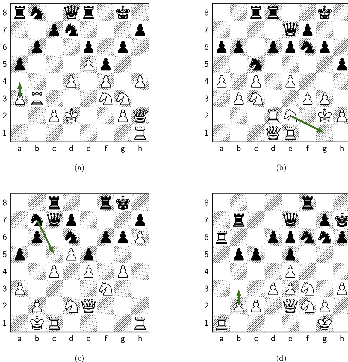
Figure 21: Move 27, White: a4. (a) Our position; Melanie plays a4 (a3a4). Panels (b)–(d) are the retrieved master positions whose correspondence most drove this move (highest QAP objective among those that transfer to it). (b) Retrieved from ccr1_top_p0002#536 (ply 64) [structural distance d=98 , QAP obj=95]: the master played Ng1; under \mu our Pa3 plays the role of that game’s Ne2 (a cross-type correspondence); cross-type roles: our Nf3 as their Qd1 , our nb8 as their Re1 ; transferred move a3a4 ( endorses this move ). (c) Retrieved from ccr1_top_p0000#1706 (ply 43) [structural distance d=96 , QAP obj=80]: the master played Nc5; under \mu our Pa3 plays the role of that game’s Nb2 (a cross-type correspondence); cross-type roles: our Nf3 as their Rc8 , our Pd4 as their Rf8 ; transferred move a3a4 ( endorses this move ). (d) Retrieved from ccr1_top_p0001#1937 (ply 46) [structural distance d=91 , QAP obj=53]: the master played b3; under \mu our Pa3 plays the role of that game’s Pb2 ; cross-type roles: our Rb3 as their Qe2 , our pe6 as their Nf2 ; transferred move a3a4 ( endorses this move ). Synthesis: 4 retrieved analogs transferred to a4 (summed QAP objective 281, the strongest correspondence among the candidate moves); Melanie committed it via the search selector.
