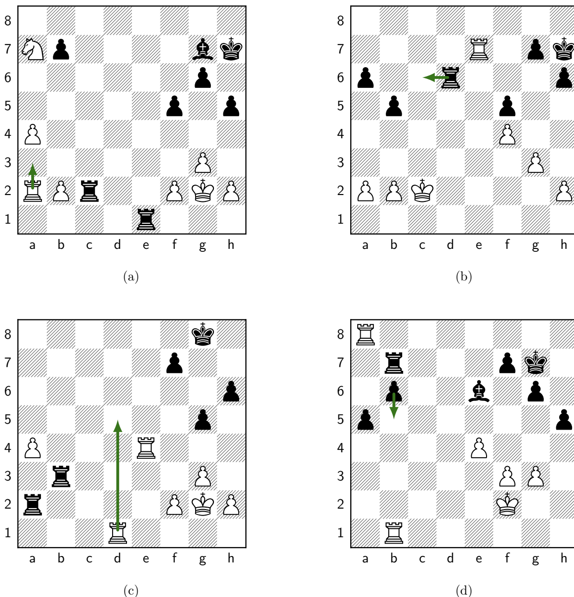
Figure 34: Move 40, White: Ra3. (a) Our position; Melanie plays Ra3 (a2a3). Panels (b)–(d) are the retrieved master positions whose correspondence most drove this move (highest QAP objective among those that transfer to it). (b) Retrieved from ccr1_top_p0002#3279 (ply 83) [structural distance d=34 , QAP obj=25]: the master played Rc6+; under \mu our Ra2 plays the role of that game’s Rd3; cross-type roles: our Na7 as their Pf5, our re1 as their pa2; transferred move a2a3 ( endorses this move ). (c) Retrieved from ccr1_top_p0002#3322 (ply 76) [structural distance d=38 , QAP obj=17]: the master played Rd5; under \mu our Ra2 plays the role of that game’s Rd1; cross-type roles: our Pa4 as their Re4, our bg7 as their pf7; transferred move a2a3 ( endorses this move ). (d) Retrieved from ccr1_top_p0001#2622 (ply 91) [structural distance d=36 , QAP obj=13]: the master played b5; under \mu our Ra2 plays the role of that game’s Pb3 (a cross-type correspondence); cross-type roles: our Na7 as their Rb7, our Pf2 as their Be6; transferred move a2a3 ( endorses this move ). Synthesis: 4 retrieved analogs transferred to Ra3 (summed QAP objective 79, the strongest correspondence among the candidate moves); Melanie committed it via the search selector.
