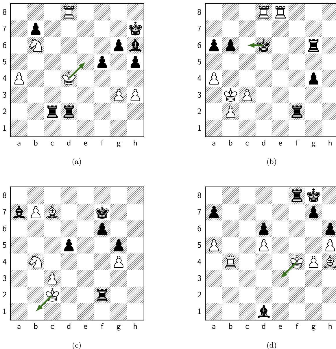
Figure 45: Move 51, White: Ke5. (a) Our position; Melanie plays Ke5 (d4e5). Panels (b)–(d) are the retrieved master positions whose correspondence most drove this move (highest QAP objective among those that transfer to it). (b) Retrieved from ccrl_top_p0000#405 (ply 117) [structural distance d=34 , QAP obj=74]: the master played Kc6; under \mu our Kd4 plays the role of that game’s Kd3; cross-type roles: our bh6 as their pc3, our Nb6 as their Rf2; transferred move d4e5 ( endorses this move ). (c) Retrieved from ccrl_top_p0000#2709 (ply 114) [structural distance d=40 , QAP obj=51]: the master played Kb1; under \mu our Kd4 plays the role of that game’s Kc2; cross-type roles: our rc2 as their Pc3, our Rd8 as their Nb4; transferred move d4e5 ( endorses this move ). (d) Retrieved from ccrl_top_p0003#991 (ply 84) [structural distance d=40 , QAP obj=42]: the master played Ke3; under \mu our Kd4 plays the role of that game’s Kf4; cross-type roles: our rc2 as their bd1, our bh6 as their Pg4; transferred move d4e5 ( endorses this move ). Synthesis: 5 retrieved analogs transferred to Ke5 (summed QAP objective 209, the strongest correspondence among the candidate moves); Melanie committed it via the search selector.
