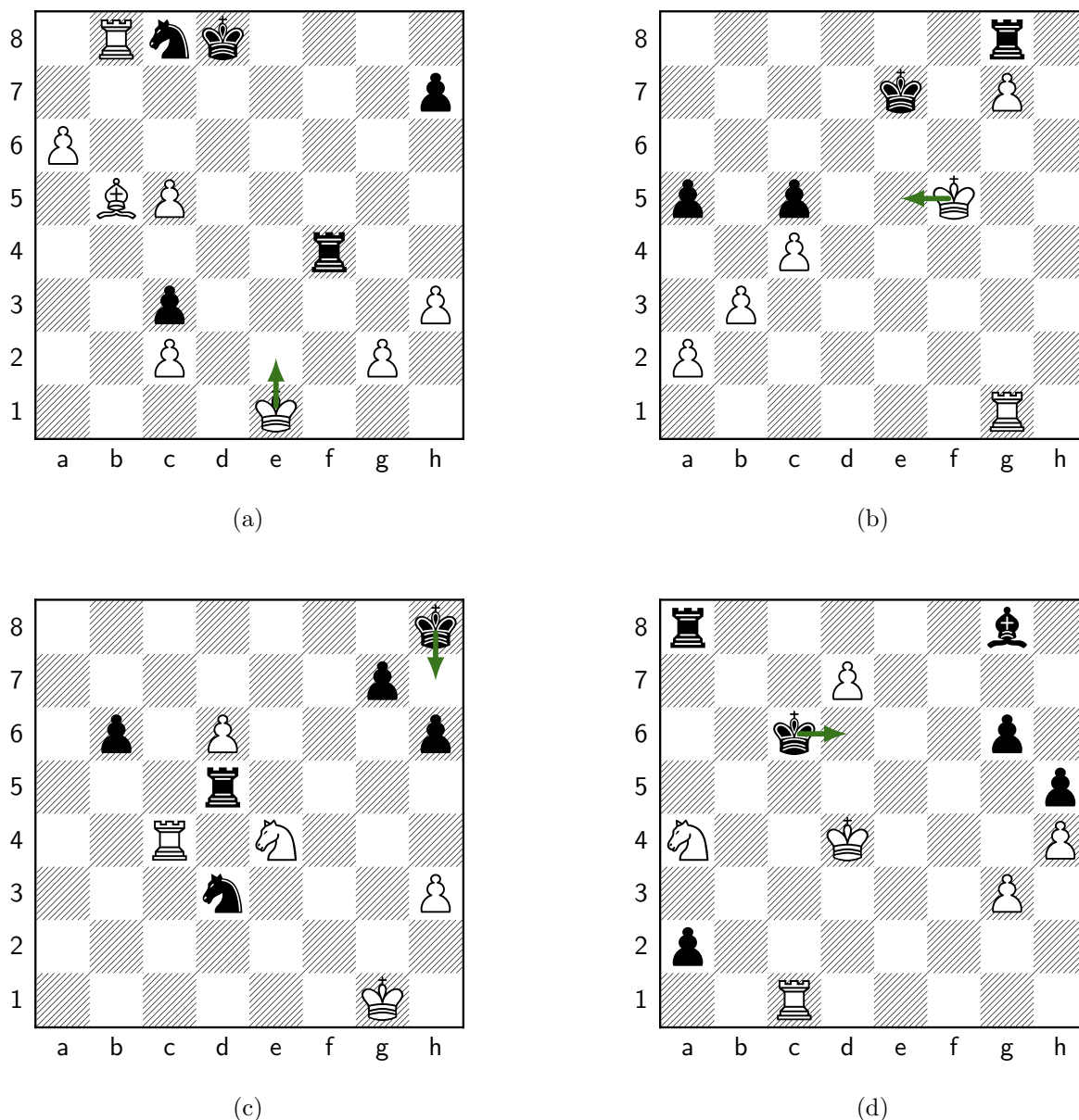
Figure 67: Move 73, White: Ke2. (a) Our position; Melanie plays Ke2 (e1e2). Panels (b)–(d) are the retrieved master positions whose correspondence most drove this move (highest QAP objective among those that transfer to it). (b) Retrieved from lichess_elite_2024-09_p0025#1463 (ply 154) [structural distance d=35 , QAP obj=14]: the master played Ke5; under \mu our Ke1 plays the role of that game’s Kf5; cross-type roles: our Bb5 as their Rg1, our rf4 as their pa5; transferred move e1e2 ( endorses this move ). (c) Retrieved from lichess_elite_2024-09_p0024#881 (ply 137) [structural distance d=37 , QAP obj=9]: the master played Kh7; under \mu our Ke1 plays the role of that game’s Kh1; cross-type roles: our nc8 as their pd6, our Pc2 as their rc4; transferred move e1e2 ( endorses this move ). (d) Retrieved from lichess_elite_2025-11_p0000#345 (ply 135) [structural distance d=29 , QAP obj=2]: the master played Kd6; under \mu our Ke1 plays the role of that game’s Kc3; transferred move e1e2 ( endorses this move ). Synthesis: 4 retrieved analogs transferred to Ke2 (summed QAP objective 27, the strongest correspondence among the candidate moves); Melanie committed it via the search selector.
