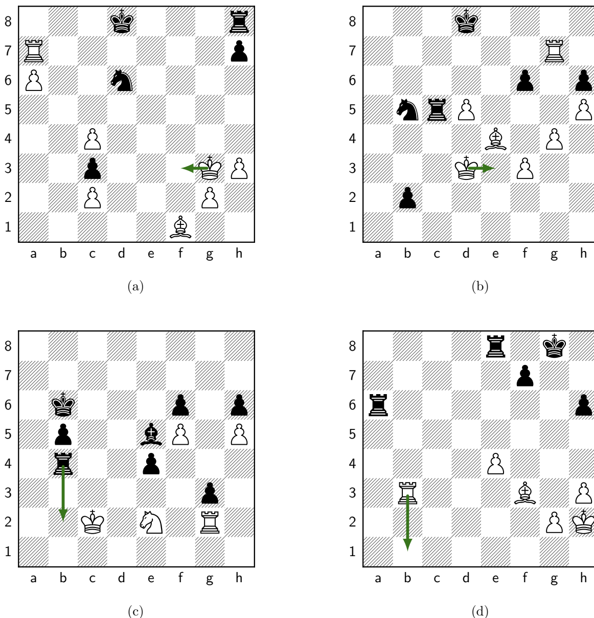
Figure 60: Move 66, White: Kf3. (a) Our position; Melanie plays Kf3 (g3f3). Panels (b)–(d) are the retrieved master positions whose correspondence most drove this move (highest QAP objective among those that transfer to it). (b) Retrieved from twic1500#281 (ply 120) [structural distance d=47 , QAP obj=12]: the master played Ke3; under \mu our Kg3 plays the role of that game's Kd3; cross-type roles: our Pg2 as their Be4, our rh8 as their nb5; transferred move g3f3 ( endorses this move ). (c) Retrieved from lichess_elite_2024-09_p0013#204 (ply 121) [structural distance d=26 , QAP obj=16]: the master played Rb2+; under \mu our Ra7 plays the role of that game's Rb5; cross-type roles: our nd6 as their rg2; transferred move a7e7. (d) Retrieved from lichess_elite_2024-09_p0012#3261 (ply 128) [structural distance d=42 , QAP obj=11]: the master played Rb1; under \mu our Ra7 plays the role of that game's Rb3; cross-type roles: our Pa6 as their ra6, our nd6 as their re8; transferred move a7g7. Synthesis: 1 retrieved analog transferred to Kf3 (summed QAP objective 12, the strongest correspondence among the candidate moves); Melanie committed it via the search selector.
