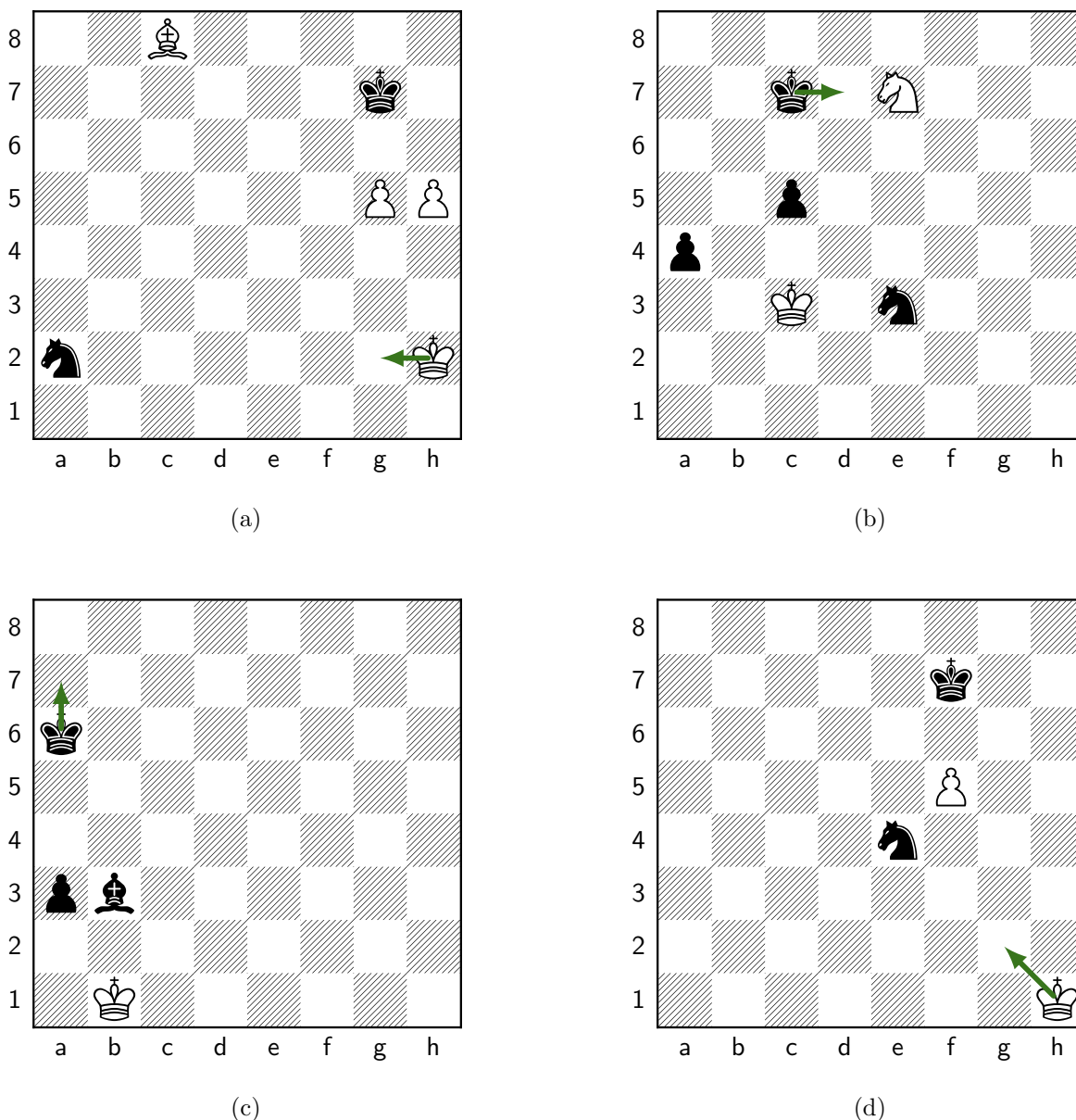
Figure 115: Move 121, White: Kg2. (a) Our position; Melanie plays Kg2 (h2g2). Panels (b)–(d) are the retrieved master positions whose correspondence most drove this move (highest QAP objective among those that transfer to it). (b) Retrieved from lichess_elite_2024-09_p0012#886 (ply 235) [structural distance d=4 , QAP obj=1]: the master played Kd7; under \mu our Kh2 plays the role of that game’s Kc2; cross-type roles: our Bc8 as their Ne3; transferred move h2g2 ( endorses this move ). (c) Retrieved from lichess_elite_2024-09_p0023#1101 (ply 239) [structural distance d=8 , QAP obj=1]: the master played Ka7; under \mu our Kh2 plays the role of that game’s Ka3; cross-type roles: our Pg5 as their Bb3; transferred move h2g2 ( endorses this move ). (d) Retrieved from lichess_elite_2024-09_p0019#3007 (ply 238) [structural distance d=8 , QAP obj=1]: the master played Kg2; under \mu our Kh2 plays the role of that game’s Kh1; transferred move h2g2 ( endorses this move ). Synthesis: 5 retrieved analogs transferred to Kg2 (summed QAP objective 3, the strongest correspondence among the candidate moves); Melanie committed it via the search selector.
