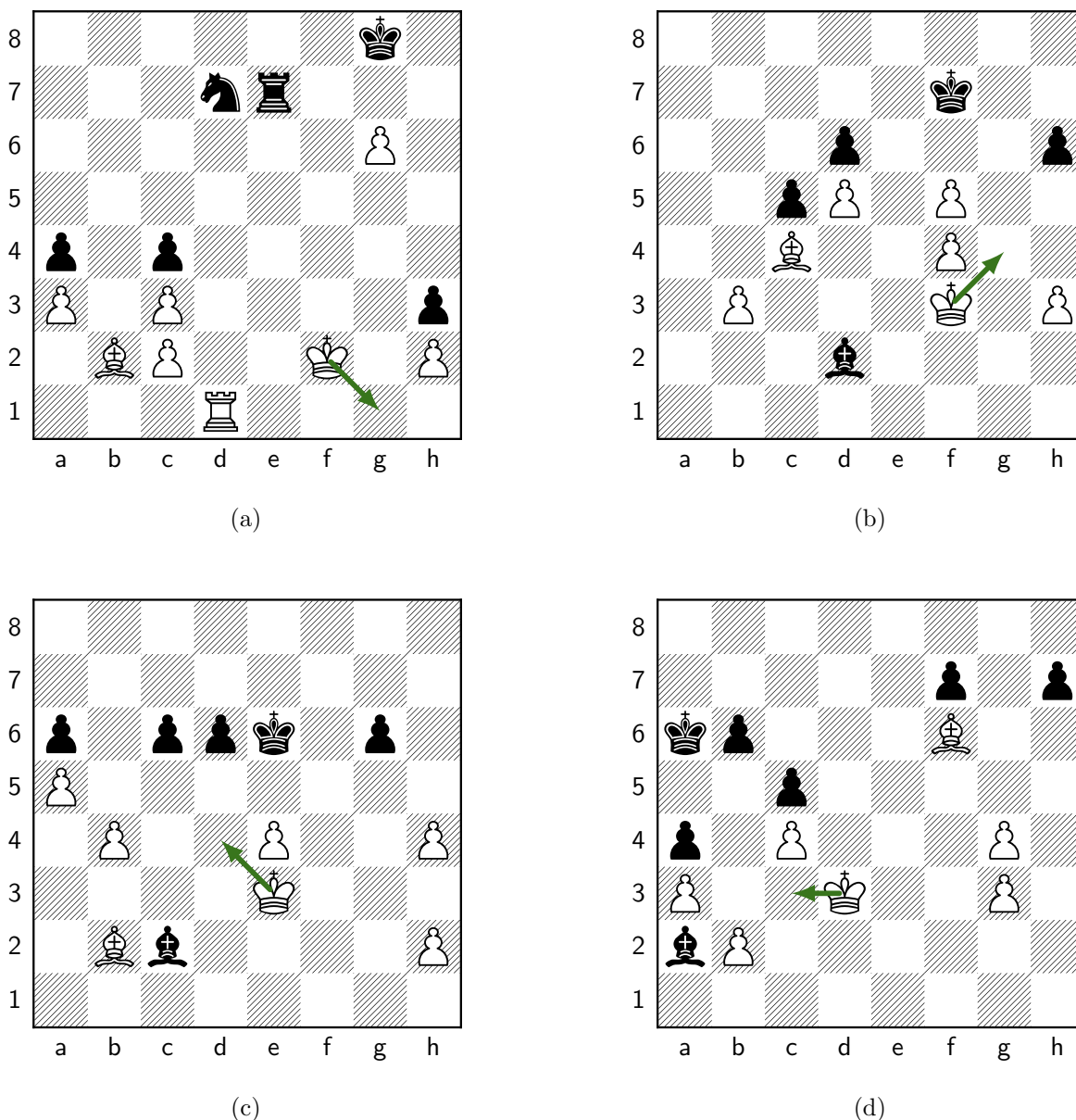
Figure 56: Move 62, White: Kg1. (a) Our position; Melanie plays Kg1 (f2g1). Panels (b)–(d) are the retrieved master positions whose correspondence most drove this move (highest QAP objective among those that transfer to it). (b) Retrieved from ccr1_top_p0003#2461 (ply 138) [structural distance d=32 , QAP obj=21]: the master played Kg4; under \mu our Kf2 plays the role of that game’s Kf3; cross-type roles: our Rd1 as their bd2, our nd7 as their Pf4; transferred move f2g1 ( endorses this move ). (c) Retrieved from ccr1_top_p0002#3048 (ply 106) [structural distance d=38 , QAP obj=20]: the master played Kd4; under \mu our Kf2 plays the role of that game’s Ke3; cross-type roles: our Pg6 as their Bb2, our Rd1 as their bc2; transferred move f2g1 ( endorses this move ). (d) Retrieved from ccr1_top_p0002#3850 (ply 108) [structural distance d=38 , QAP obj=20]: the master played Kc3; under \mu our Kf2 plays the role of that game’s Kd3; cross-type roles: our Rd1 as their ba2, our nd7 as their Pc4; transferred move f2g1 ( endorses this move ). Synthesis: 11 retrieved analogs transferred to Kg1 (summed QAP objective 132, the strongest correspondence among the candidate moves); Melanie committed it via the search selector.
