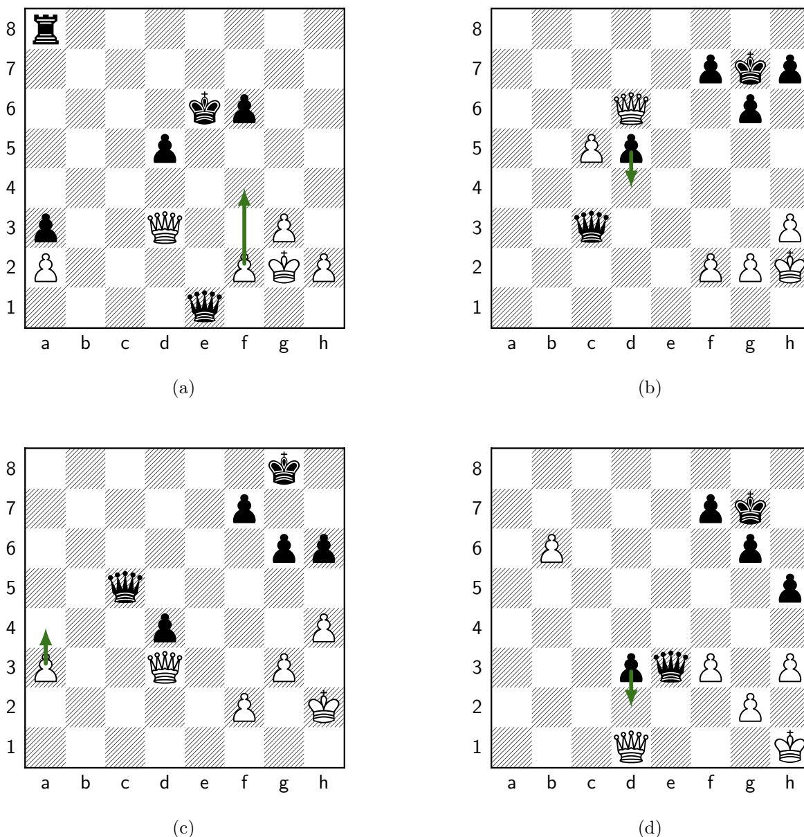
Figure 31: Move 40, White: f4. (a) Our position; Melanie plays f4 (f2f4). Panels (b)–(d) are the retrieved master positions whose correspondence most drove this move (highest QAP objective among those that transfer to it). (b) Retrieved from lichess_elite_2024-09_p0031#3668 (ply 77) [structural distance d=23 , QAP obj=35]: the master played d4; under \mu our Pf2 plays the role of that game’s Pd4; transferred move f2f4 ( endorses this move ). (c) Retrieved from lichess_elite_2024-09_p0030#2721 (ply 88) [structural distance d=23 , QAP obj=33]: the master played a4; under \mu our Pf2 plays the role of that game’s Pa3; cross-type roles: our ra8 as their ph6; transferred move f2f4 ( endorses this move ). (d) Retrieved from lichess_elite_2024-09_p0013#1614 (ply 83) [structural distance d=18 , QAP obj=33]: the master played d2; under \mu our Pf2 plays the role of that game’s Pd6; cross-type roles: our ra8 as their ph3; transferred move f2f4 ( endorses this move ). Synthesis: 5 retrieved analogs transferred to f4 (summed QAP objective 145, the strongest correspondence among the candidate moves); Melanie committed it via the search selector.
