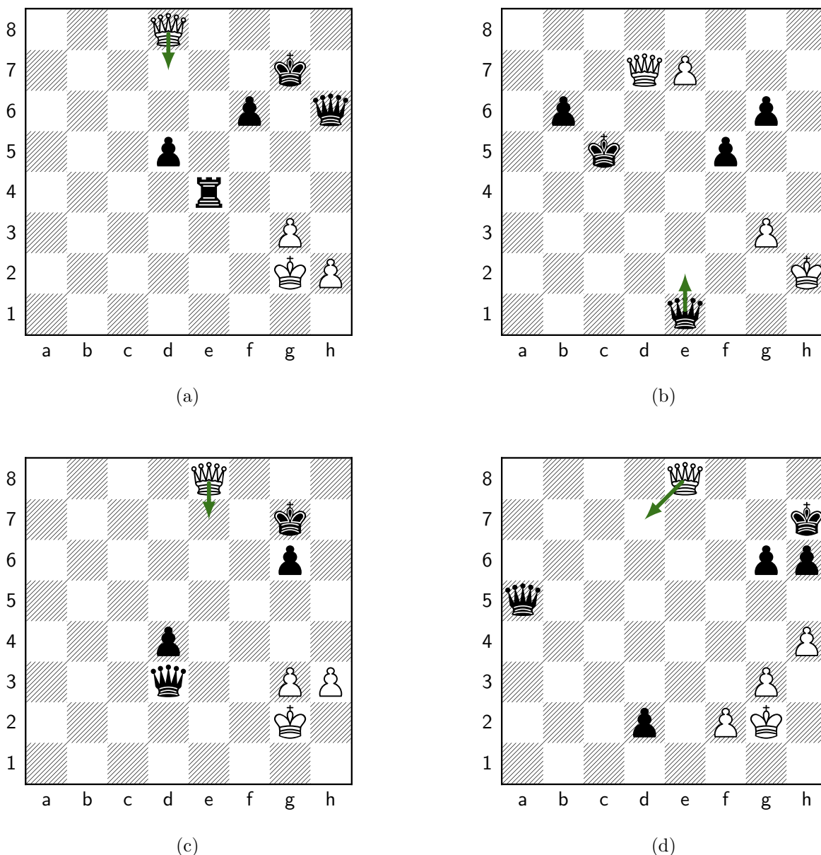
Figure 60: Move 69, White: Qd7+. (a) Our position; Melanie plays Qd7+ (d8d7). Panels (b)–(d) are the retrieved master positions whose correspondence most drove this move (highest QAP objective among those that transfer to it). (b) Retrieved from lichess_elite_2024-09_p0020#729 (ply 125) [structural distance d=20 , QAP obj=40]: the master played Qe2+; under \mu our Qd8 plays the role of that game’s Qe8; cross-type roles: our re4 as their Pb6; transferred move d8d7 ( endorses this move ). (c) Retrieved from lichess_elite_2024-09_p0031#3671 (ply 126) [structural distance d=28 , QAP obj=32]: the master played Qe7+; under \mu our Qd8 plays the role of that game’s Qe8; cross-type roles: our re4 as their Ph3; transferred move d8d7 ( endorses this move ). (d) Retrieved from lichess_elite_2024-09_p0030#2721 (ply 122) [structural distance d=32 , QAP obj=20]: the master played Qd7+; under \mu our Qd8 plays the role of that game’s Qe8; cross-type roles: our re4 as their pd2; transferred move d8d7 ( endorses this move ). Synthesis: 8 retrieved analogs transferred to Qd7+ (summed QAP objective 195, the strongest correspondence among the candidate moves); Melanie committed it via the search selector.
