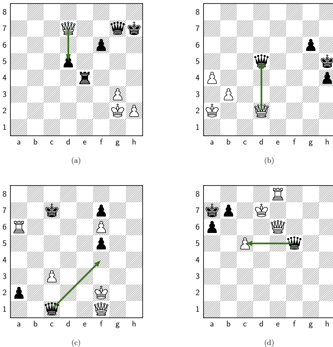
Figure 63: Move 72, White: Qxd5. (a) Our position; Melanie plays Qxd5 (d7d5). Panels (b)–(d) are the retrieved master positions whose correspondence most drove this move (highest QAP objective among those that transfer to it). (b) Retrieved from lichess_elite_2024-09_p0022#83 (ply 140) [structural distance d=31 , QAP obj=48]: the master played Qxd5+; under \mu our Qd7 plays the role of that game’s Qd2; cross-type roles: our re4 as their ph4; transferred move d7d5 ( endorses this move ). (c) Retrieved from lichess_elite_2024-09_p0018#90 (ply 149) [structural distance d=31 , QAP obj=46]: the master played Qf4+; under \mu our Qd7 plays the role of that game’s Qc8; cross-type roles: our pf6 as their ra6, our re4 as their Pf5; transferred move d7d5 ( endorses this move ). (d) Retrieved from lichess_elite_2024-09_p0031#193 (ply 129) [structural distance d=21 , QAP obj=35]: the master played Qxc5; under \mu our Qd7 plays the role of that game’s Qf4; cross-type roles: our pf6 as their re8; transferred move d7d5 ( endorses this move ). Synthesis: 6 retrieved analogs transferred to Qxd5 (summed QAP objective 165, the strongest correspondence among the candidate moves); Melanie committed it via the search selector.
