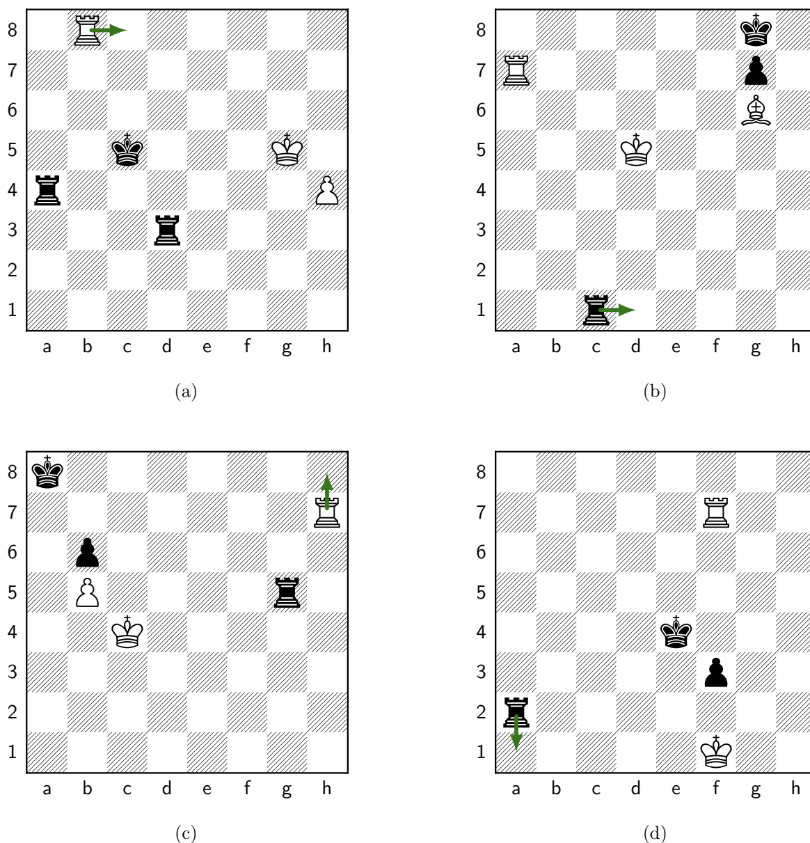
Figure 81: Move 87, White: Rc8+. (a) Our position; Melanie plays Rc8+ (b8c8). Panels (b)–(d) are the retrieved master positions whose correspondence most drove this move (highest QAP objective among those that transfer to it). (b) Retrieved from ccr1_top_p0003#1855 (ply 159) [structural distance d=5 , QAP obj=19]: the master played Rd1+; under \mu our Rb8 plays the role of that game's Rc8; cross-type roles: our rd3 as their bg6; transferred move b8c8 ( endorses this move ). (c) Retrieved from ccr1_top_p0000#3255 (ply 156) [structural distance d=6 , QAP obj=15]: the master played Rh8+; under \mu our Rb8 plays the role of that game's Rh7; cross-type roles: our rd3 as their pb6; transferred move b8c8 ( endorses this move ). (d) Retrieved from ccr1_top_p0000#139 (ply 171) [structural distance d=6 , QAP obj=12]: the master played Ra1+; under \mu our Rb8 plays the role of that game's Ra7; transferred move b8c8 ( endorses this move ). Synthesis: 3 retrieved analogs transferred to Rc8+ (summed QAP objective 46, the strongest correspondence among the candidate moves); Melanie committed it via the search selector.
