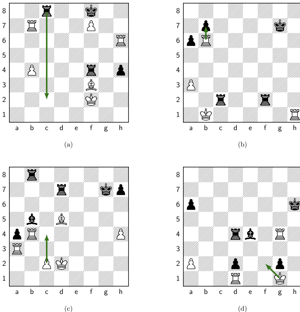
Figure 40: Move 46, Black: Rc2+. (a) Our position; Melanie plays Rc2+ (c8c2). Panels (b)–(d) are the retrieved master positions whose correspondence most drove this move (highest QAP objective among those that transfer to it). (b) Retrieved from ccr1_top_p0001#3551 (ply 96) [structural distance d=33 , QAP obj=3]: the master played Rxb7+; under \mu our Rc1 plays the role of that game’s Rb6; cross-type roles: our pf7 as their rc2, our rh6 as their Pa3; transferred move c8c2 ( endorses this move ). (c) Retrieved from ccr1_top_p0003#1322 (ply 74) [structural distance d=34 , QAP obj=54]: the master played c4; under \mu our Rc1 plays the role of that game’s Pc2 (a cross-type correspondence); cross-type roles: our Kf8 as their Ra3, our rb7 as their ph7; transferred move c8c3. (d) Retrieved from ccr1_top_p0003#2780 (ply 88) [structural distance d=17 , QAP obj=37]: the master played Kf2; under \mu our Kf1 plays the role of that game’s Kg1; cross-type roles: our rh6 as their pa6; transferred move f8g7. Synthesis: 1 retrieved analog transferred to Rc2+ (summed QAP objective 3, the strongest correspondence among the candidate moves); Melanie committed it via the search selector.
