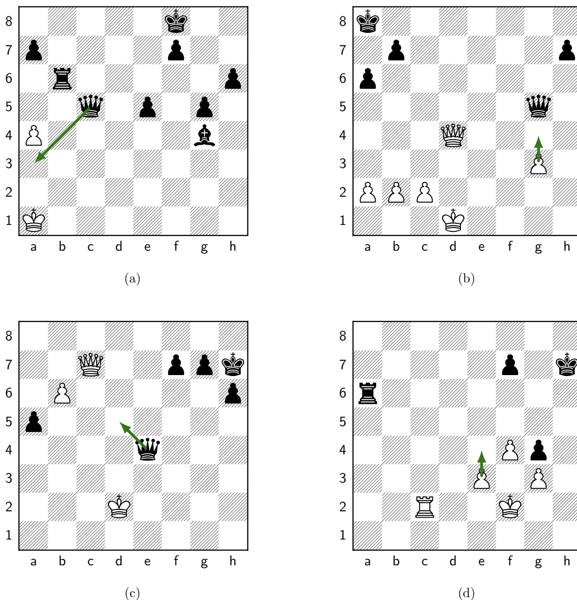
Figure 33: Move 42, Black: Qa3#. (a) Our position; Melanie plays Qa3# (c5a3). Panels (b)–(d) are the retrieved master positions whose correspondence most drove this move (highest QAP objective among those that transfer to it). (b) Retrieved from ccr1_top_p0002#541 (ply 72) [structural distance d=48 , QAP obj=3]: the master played g4; under \mu our Ph3 plays the role of that game’s Pg3 ; cross-type roles: our Pg5 as their qg5 , our Rb6 as their pa6 ; transferred move h6h5. (c) Retrieved from ccr1_top_p0003#416 (ply 75) [structural distance d=45 , QAP obj=2]: the master played Qd5+; under \mu our Qc4 plays the role of that game’s Qe5 ; cross-type roles: our Rb6 as their qc7 ; transferred move c5d5. (d) Retrieved from ccr1_top_p0001#2701 (ply 86) [structural distance d=45 , QAP obj=2]: the master played e4; under \mu our Pf2 plays the role of that game’s Pe3 ; cross-type roles: our Qc5 as their Rc2 , our Bg4 as their Pf4 ; transferred move f7f5. Synthesis: no retrieved analog transferred to Qa3# – the search selector chose it on value (material / mate); panels (b)–(d) show the strongest nearby analogies.
