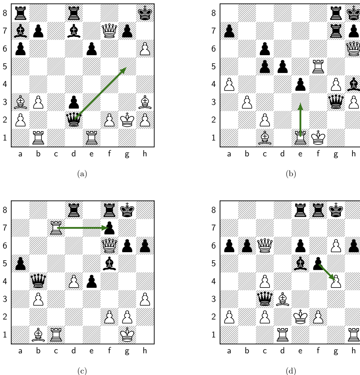
Figure 27: Move 33, Black: Qg5+. (a) Our position; Melanie plays Qg5+ (d2g5). Panels (b)–(d) are the retrieved master positions whose correspondence most drove this move (highest QAP objective among those that transfer to it). (b) Retrieved from lichess_elite_2025-11_p0000#2140 (ply 56) [structural distance d=104 , QAP obj=88]: the master played Re3 ; under \mu our Bd2 plays the role of that game's Re1 (a cross-type correspondence); cross-type roles: our Pd3 as their Bc1 , our Ba7 as their Ph3 ; transferred move d7c6 . (c) Retrieved from lichess_elite_2024-09_p0023#3757 (ply 66) [structural distance d=81 , QAP obj=69]: the master played Rxf7 ; under \mu our Ba2 plays the role of that game's Rc7 (a cross-type correspondence); cross-type roles: our ph2 as their Rc1 , our qf7 as their Pf2 ; transferred move a7f2 . (d) Retrieved from lichess_elite_2024-09_p0020#2177 (ply 53) [structural distance d=85 , QAP obj=62]: the master played fxf4 ; under \mu our Pe3 plays the role of that game's Pf4 ; cross-type roles: our Bd7 as their Re8 , our Ba7 as their Pa6 ; transferred move e6e5 . Synthesis: no retrieved analog transferred to Qg5+ – the search selector chose it on value (material / mate); panels (b)–(d) show the strongest nearby analogies.
