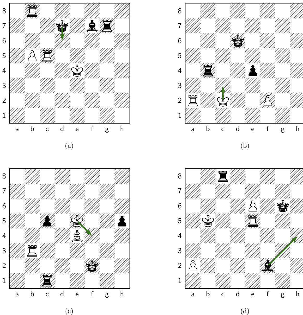
Figure 80: Move 86, Black: Kd6 . (a) Our position; Melanie plays Kd6 (d7d6). Panels (b)–(d) are the retrieved master positions whose correspondence most drove this move (highest QAP objective among those that transfer to it). (b) Retrieved from ccr1_top_p0001#1233 (ply 174) [structural distance d=15 , QAP obj=2]: the master played Kc3; under \mu our Kd2 plays the role of that game’s Kc2; cross-type roles: our Bf7 as their Pf2, our rc5 as their pe4; transferred move d7d6 ( endorses this move ). (c) Retrieved from ccr1_top_p0001#3038 (ply 176) [structural distance d=14 , QAP obj=2]: the master played Kf4; under \mu our Kd2 plays the role of that game’s Ke5; cross-type roles: our Bf7 as their rc1, our rc5 as their Be4; transferred move d7d6 ( endorses this move ). (d) Retrieved from ccr1_top_p0000#3103 (ply 155) [structural distance d=12 , QAP obj=2]: the master played Bh4; under \mu our Bf2 plays the role of that game’s Bf7; cross-type roles: our Rg7 as their pa2; transferred move f7b3. Synthesis: 2 retrieved analogs transferred to Kd6 (summed QAP objective 4, the strongest correspondence among the candidate moves); Melanie committed it via the search selector.
