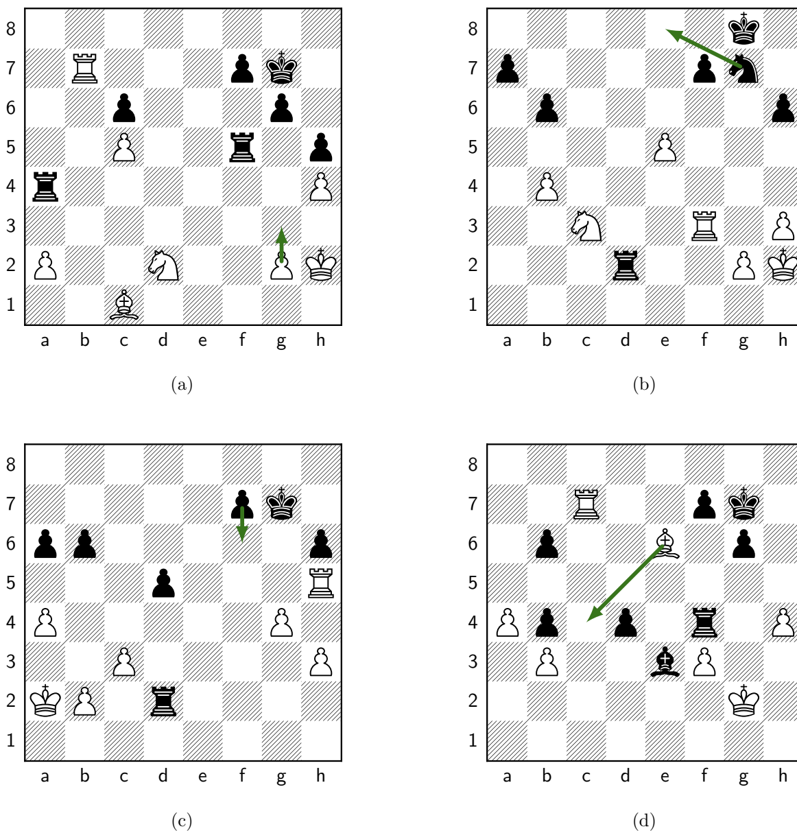
Figure 25: Move 31, White: g3. (a) Our position; Melanie plays g3 (g2g3). Panels (b)–(d) are the retrieved master positions whose correspondence most drove this move (highest QAP objective among those that transfer to it). (b) Retrieved from ccr1_top_p0003#1993 (ply 73) [structural distance d=41 , QAP obj=39]: the master played Ne8; under \mu our Pg2 plays the role of that game’s Ng2 (a cross-type correspondence); cross-type roles: our Nd2 as their Pa7, our ra4 as their Pb6; transferred move g2g3 ( endorses this move ). (c) Retrieved from ccr1_top_p0002#2617 (ply 77) [structural distance d=42 , QAP obj=28]: the master played f6; under \mu our Pg2 plays the role of that game’s Pf2; cross-type roles: our rf5 as their Pb6, our Nd2 as their pg4; transferred move g2g3 ( endorses this move ). (d) Retrieved from ccr1_top_p0003#1703 (ply 76) [structural distance d=42 , QAP obj=22]: the master played Bc4; under \mu our Pg2 plays the role of that game’s Be6 (a cross-type correspondence); cross-type roles: our Nd2 as their Pb3, our pg6 as their be3; transferred move g2g3 ( endorses this move ). Synthesis: 5 retrieved analogs transferred to g3 (summed QAP objective 114, the strongest correspondence among the candidate moves); Melanie committed it via the search selector.
