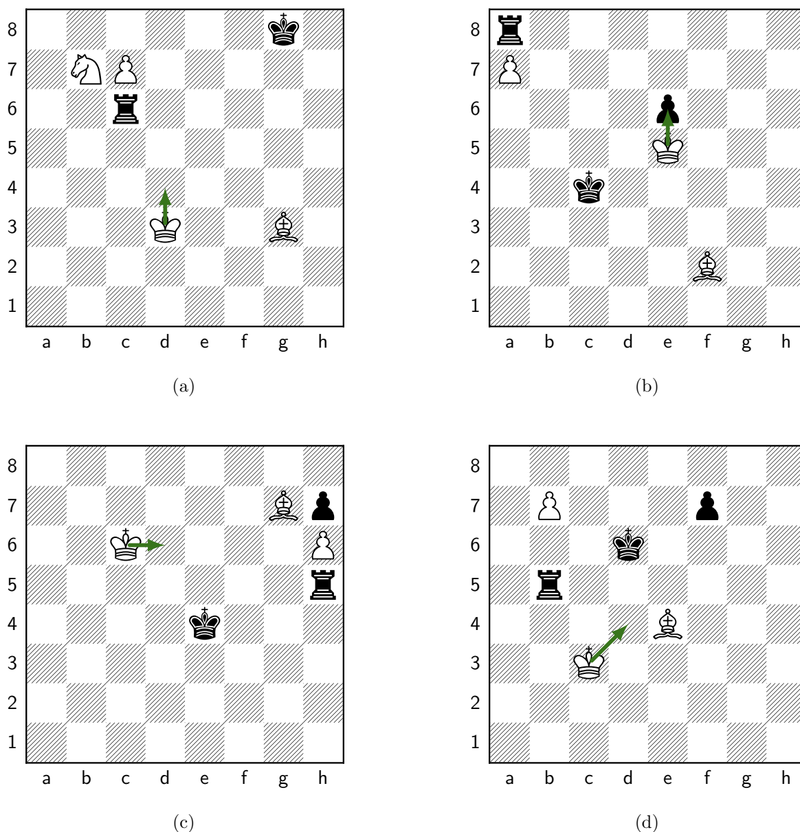
Figure 75: Move 81, White: Kd4. (a) Our position; Melanie plays Kd4 (d3d4). Panels (b)–(d) are the retrieved master positions whose correspondence most drove this move (highest QAP objective among those that transfer to it). (b) Retrieved from ccr1_top_p0000#2062 (ply 152) [structural distance d=9 , QAP obj=21]: the master played Kxe6; under \mu our Kd3 plays the role of that game’s Ke5; cross-type roles: our Nb7 as their pe6; transferred move d3d4 ( endorses this move ). (c) Retrieved from ccr1_top_p0001#2574 (ply 164) [structural distance d=9 , QAP obj=20]: the master played Kd6; under \mu our Kd3 plays the role of that game’s Kc6; cross-type roles: our Nb7 as their ph7; transferred move d3d4 ( endorses this move ). (d) Retrieved from ccr1_top_p0003#487 (ply 160) [structural distance d=3 , QAP obj=13]: the master played Kd4; under \mu our Kd3 plays the role of that game’s Kc3; cross-type roles: our Nb7 as their pf7; transferred move d3d4 ( endorses this move ). Synthesis: 8 retrieved analogs transferred to Kd4 (summed QAP objective 80, the strongest correspondence among the candidate moves); Melanie committed it via the search selector.
