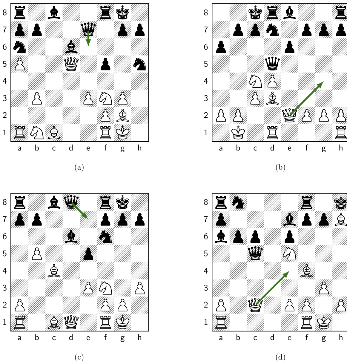
Figure 9: Move 15, Black: Qe6. (a) Our position; Melanie plays Qe6 (e7e6). Panels (b)–(d) are the retrieved master positions whose correspondence most drove this move (highest QAP objective among those that transfer to it). (b) Retrieved from ccl1_top_p0001#2817 (ply 32) [structural distance d=74 , QAP obj=41]: the master played Qg4; under \mu our Qe2 plays the role of that game’s Qe2; cross-type roles: our Nh5 as their Pb2, our ra1 as their Bd3; transferred move e7e6 ( endorses this move ). (c) Retrieved from ccl1_top_p0001#1365 (ply 27) [structural distance d=74 , QAP obj=33]: the master played Qe7; under \mu our Qe2 plays the role of that game’s Qd1; cross-type roles: our Na6 as their Bc8, our Bc8 as their Pb7; transferred move e7e6 ( endorses this move ). (d) Retrieved from ccl1_top_p0002#1590 (ply 32) [structural distance d=85 , QAP obj=33]: the master played Qe4; under \mu our Qe2 plays the role of that game’s Qc2; cross-type roles: our Bc8 as their Pa2, our Na6 as their Bf4; transferred move e7e6 ( endorses this move ). Synthesis: 7 retrieved analogs transferred to Qe6 (summed QAP objective 209, the strongest correspondence among the candidate moves); Melanie committed it via the search selector.
