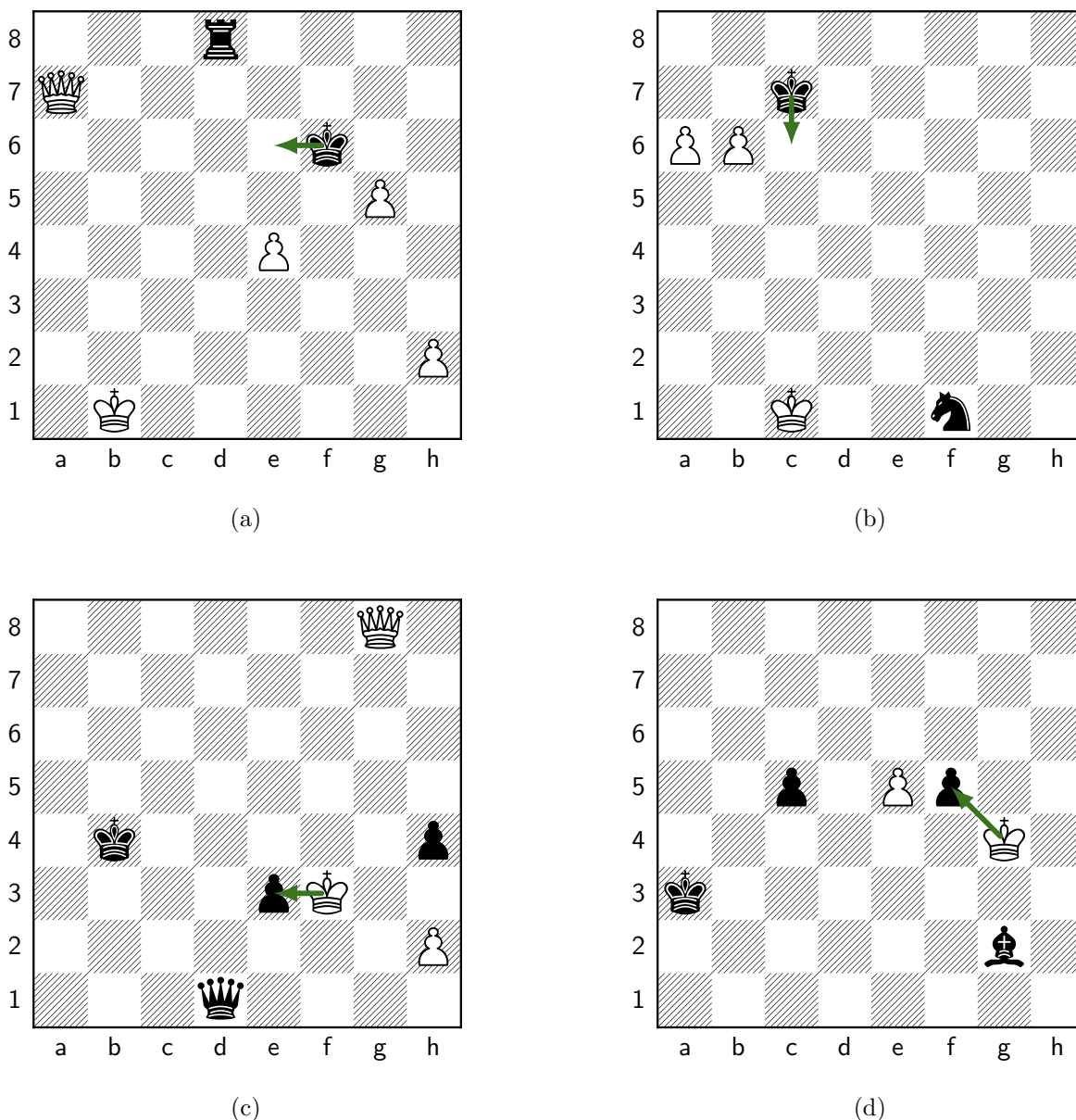
Figure 50: Move 56, Black: Ke6 . (a) Our position; Melanie plays Ke6 (f6e6). Panels (b)–(d) are the retrieved master positions whose correspondence most drove this move (highest QAP objective among those that transfer to it). (b) Retrieved from lichess_elite_2024-09_p0024#1897 (ply 95) [structural distance d=10 , QAP obj=68]: the master played Kc6; under \mu our Kf3 plays the role of that game’s Kc2; cross-type roles: our Rd8 as their Nf1; transferred move f6e6 ( endorses this move ). (c) Retrieved from lichess_elite_2024-09_p0020#899 (ply 118) [structural distance d=9 , QAP obj=36]: the master played Kxe3; under \mu our Kf3 plays the role of that game’s Kf3; cross-type roles: our pg5 as their qd1, our Rd8 as their Ph2; transferred move f6e6 ( endorses this move ). (d) Retrieved from lichess_elite_2024-09_p0024#2636 (ply 124) [structural distance d=9 , QAP obj=68]: the master played Kxf5; under \mu our Kf3 plays the role of that game’s Kg4; cross-type roles: our qa7 as their bg2, our Rd8 as their Pe5; transferred move f6e5. Synthesis: 2 retrieved analogs transferred to Ke6 (summed QAP objective 104, the strongest correspondence among the candidate moves); Melanie committed it via the search selector.
