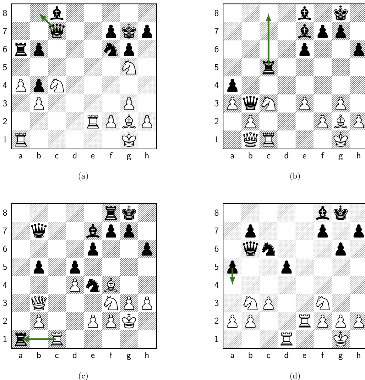
Figure 20: Move 27, Black: Qb8. (a) Our position; Melanie plays Qb8 (c7b8). Panels (b)–(d) are the retrieved master positions whose correspondence most drove this move (highest QAP objective among those that transfer to it). (b) Retrieved from ccrl_top_p0000#2982 (ply 51) [structural distance d=92 , QAP obj=43]: the master played Rc8; under \mu our Qc2 plays the role of that game’s Rc4 (a cross-type correspondence); cross-type roles: our Ra6 as their Be8, our Ph7 as their Be7; transferred move c7b8 ( endorses this move ). (c) Retrieved from ccrl_top_p0003#1112 (ply 48) [structural distance d=83 , QAP obj=32]: the master played Rxa1; under \mu our Qc2 plays the role of that game’s Rc1 (a cross-type correspondence); cross-type roles: our nc4 as their ra1, our Ra6 as their Qb3; transferred move c7b8 ( endorses this move ). (d) Retrieved from ccrl_top_p0001#2980 (ply 39) [structural distance d=68 , QAP obj=63]: the master played a4; under \mu our Pb3 plays the role of that game’s Pa4; cross-type roles: our Ra6 as their Bf8, our bg2 as their Pb7; transferred move b6b5. Synthesis: 2 retrieved analogs transferred to Qb8 (summed QAP objective 75, the strongest correspondence among the candidate moves); Melanie committed it via the search selector.
